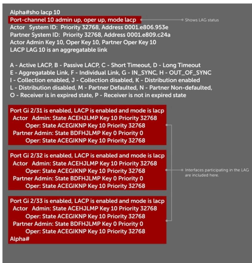
Figure 69. Verifying LAG 10 Status on ALPHA Using the show lacp Command
