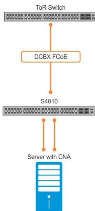
Figure 40. Configuration Example: FIP Snooping on a Switch
