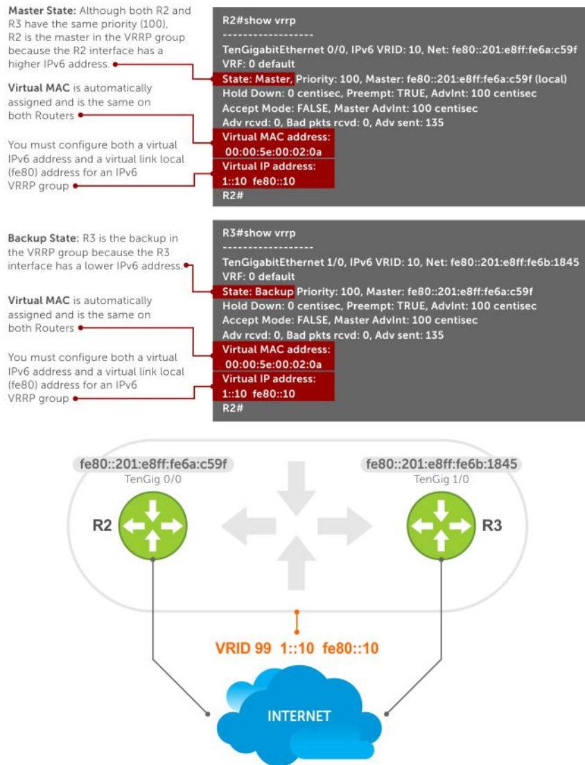
Figure 156. VRRP for IPv6 Topology
