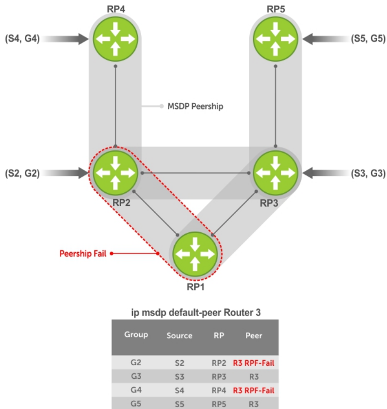
Figure 91. MSDP Default Peer, Scenario 2
