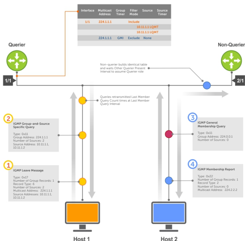
Figure 49. Membership Queries: Leaving and Staying
