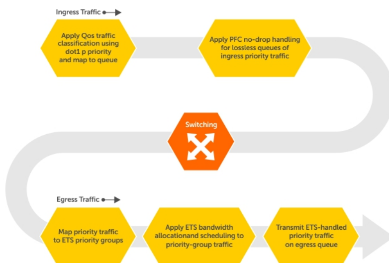
Figure 32. DCB PFC and ETS Traffic Handling
