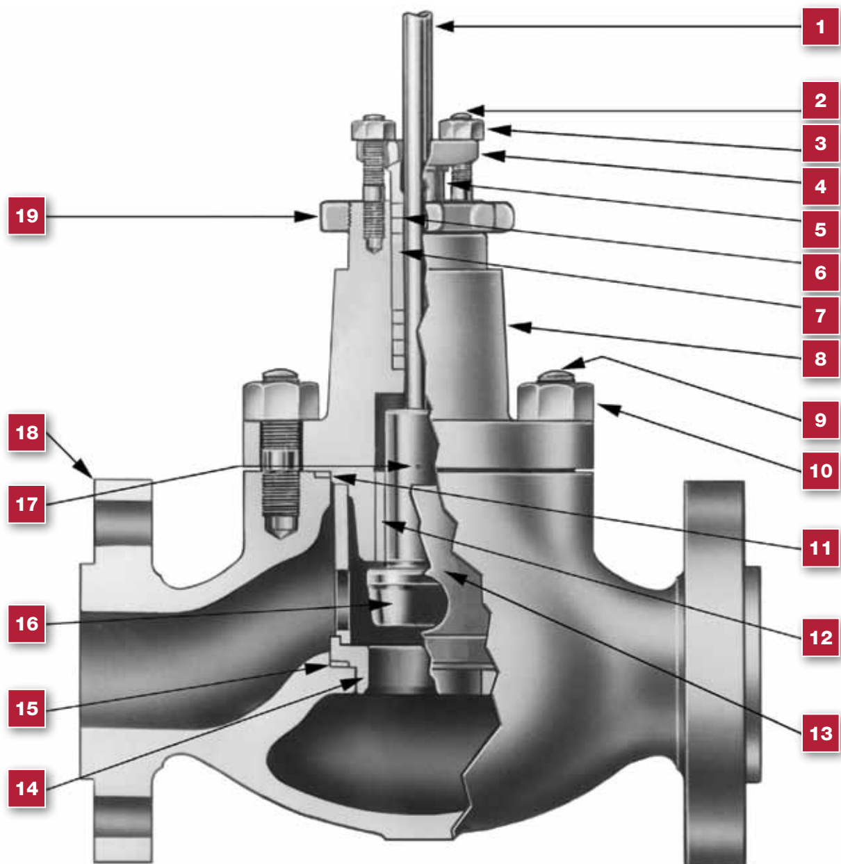
Standard Construction
