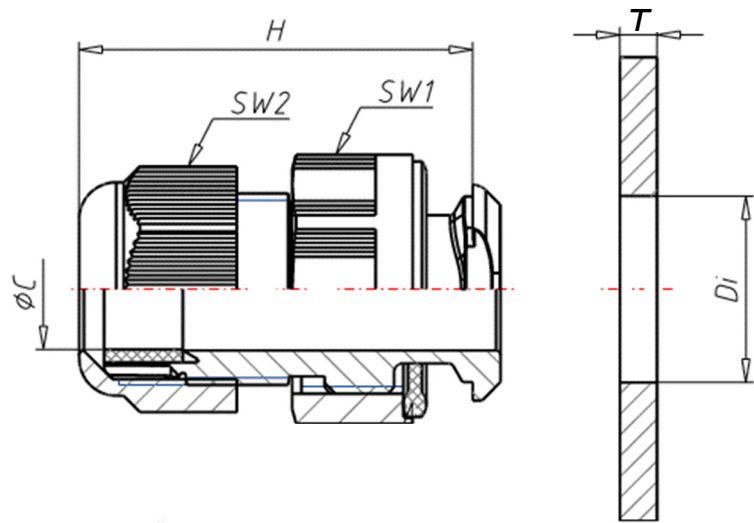
Figure 3 Mechanical Drawing, Gland Nut
