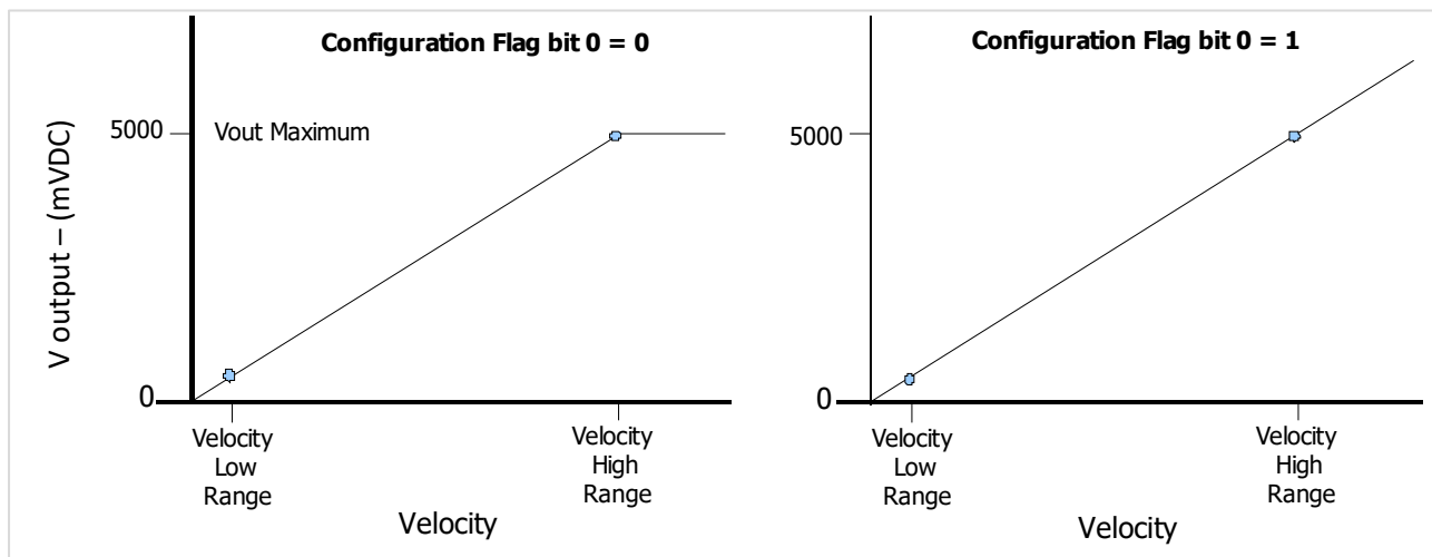
Figure 27 Velocity Analog Output: Voutput (0 – 5V) with and without Clamping
