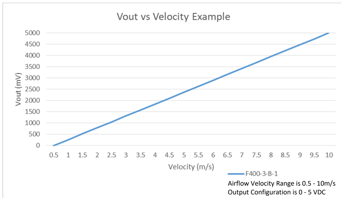
Figure 30 Velocity Analog Output: Vout vs Velocity Example
