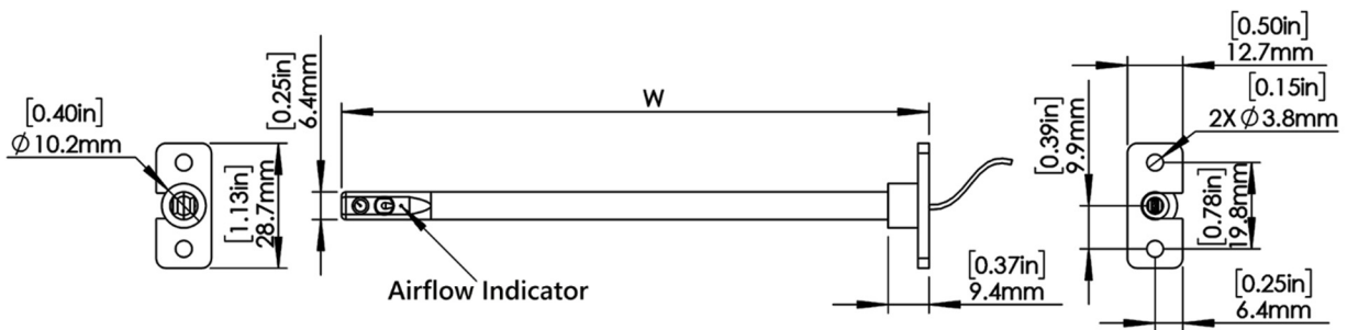
Figure 9 Wand Sensor Head (Compatible with Gland Nut HA1203)
