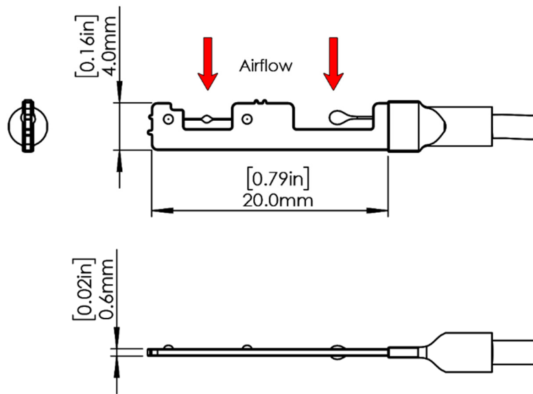
Figure 10 XS (Extra Small) Sensor Head
