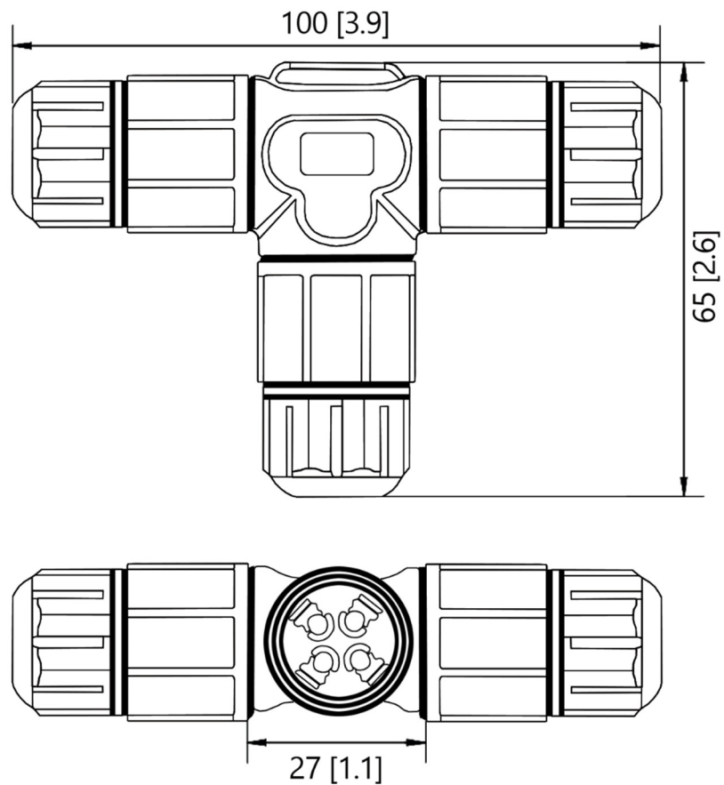
Figure 5 Mechanical Drawing, Wiring Box
