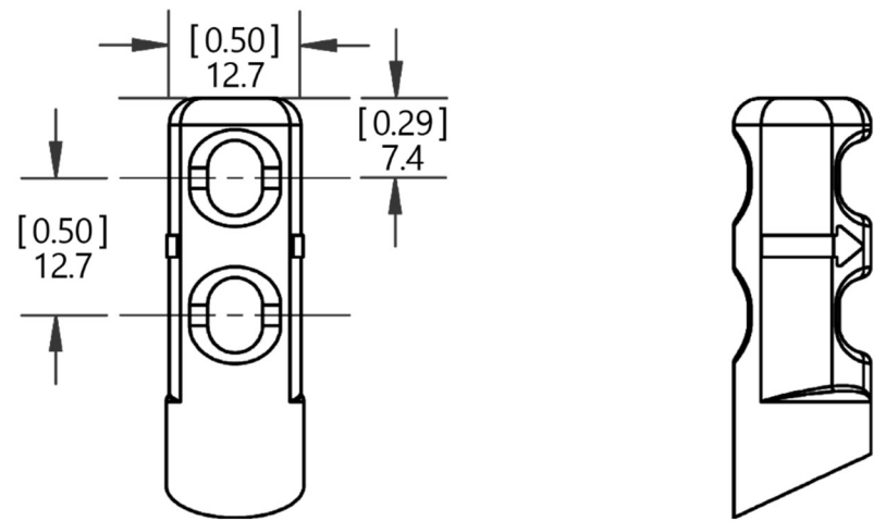
Figure 2 Mechanical Drawing, F-Series Sensor Head (Directional)
