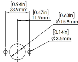
Figure 25 Wall 2 Mounting
