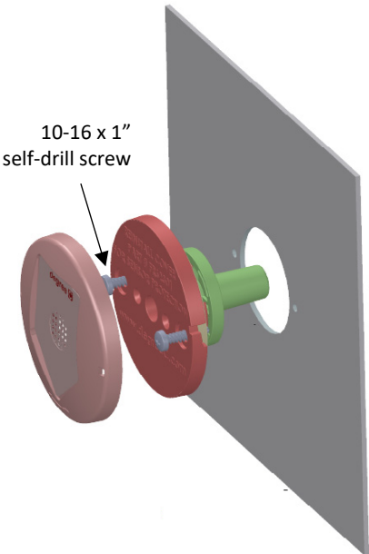
Figure 20 Sidewall Sensor Mounting - Single Walled Cabinet
