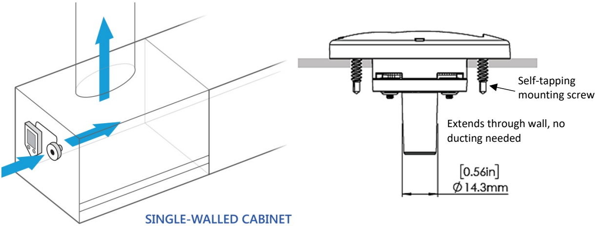
Figure 19 Sidewall Sensor on Single Walled Cabinet
