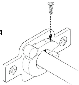
Figure 17 °C Clamp Installation
