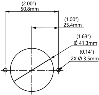
Figure 21 Sidewall Sensor Mounting Dimensions
