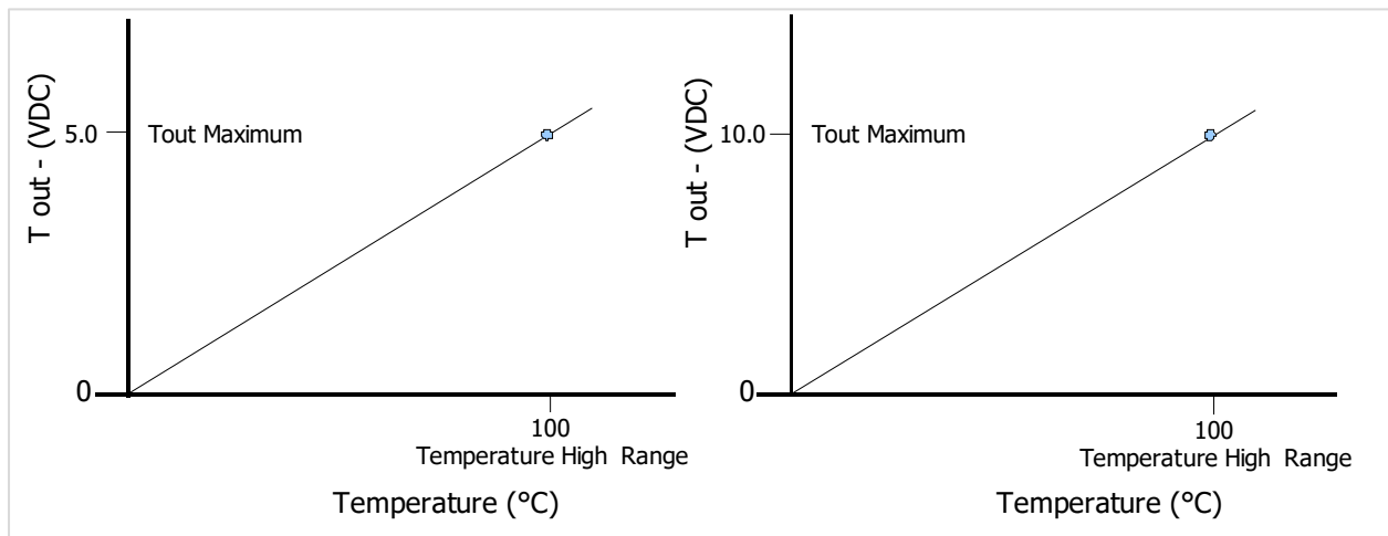
Figure 33 Temperature Analog Output: Toutput for (0 – 5V) and (0 – 10V)
