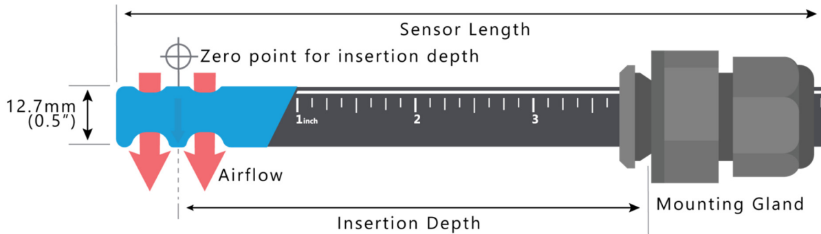
Figure 12 Probe-Style Sensor Dimensions
