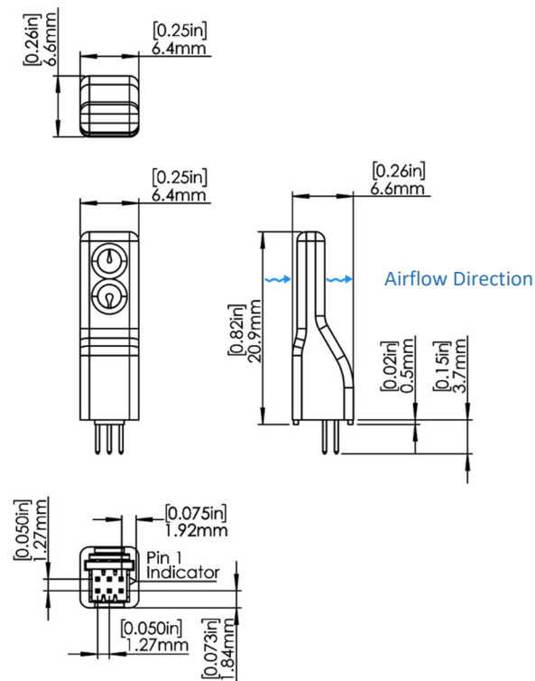
Figure 11 RF5300 Board Mount Sensor Head, PCB Sensor
