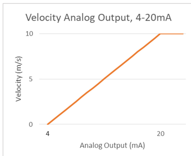
Figure 31 Velocity Analog Output: 4-20 mA Example
