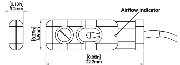
Figure 8 PC (Plastic Cap) Sensor Head
