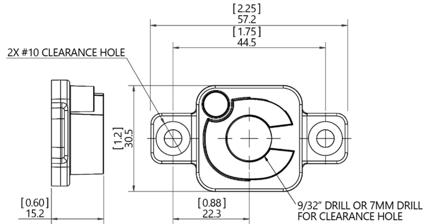
Figure 4 Mechanical Drawing, °C Clamp
