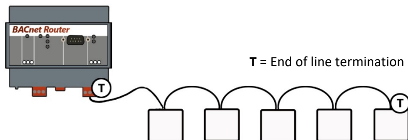
Figure 1 BACnet® MS/TP Network
