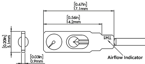
Figure 7 LP (Low Profile) Sensor Head
