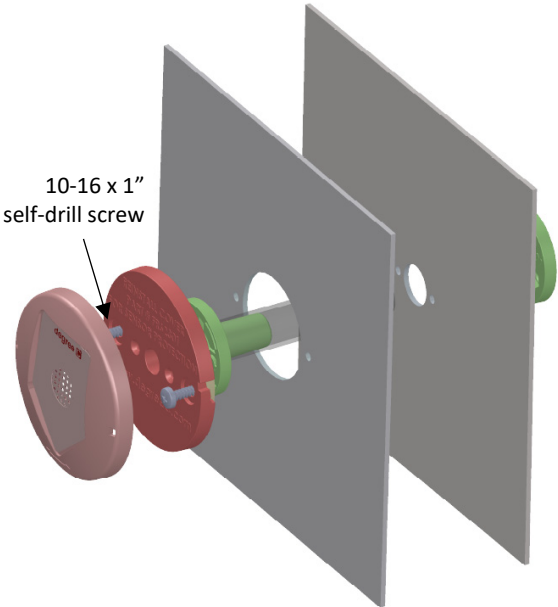
Figure 23 Sidewall Sensor Mounting - Dual Walled Cabinet
