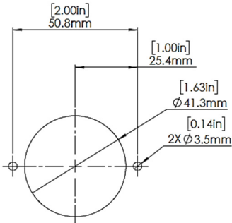
Figure 24 Wall 1 Mounting
