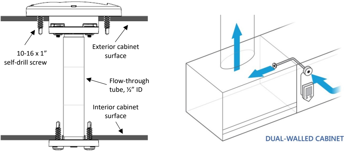
Figure 22 Sidewall Sensor on Dual Walled Cabinet
