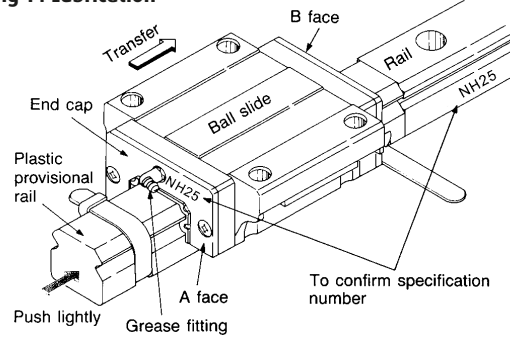
Fig 14 Lubrication
