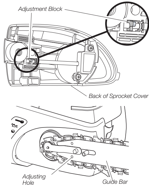
Figure 17 - Adjustment Block and Adjusting Hole Location
