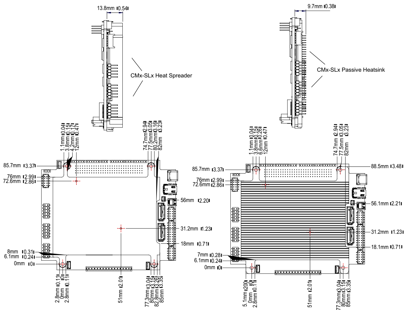
Figure 1-4: Passive Heatsink and Heat Spreader mounting dimensions (top side)
