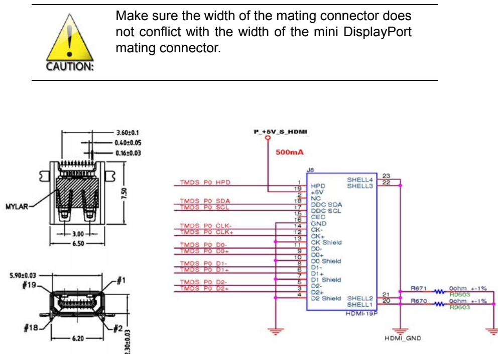
Figure 2-6: Micro HDMI connector
