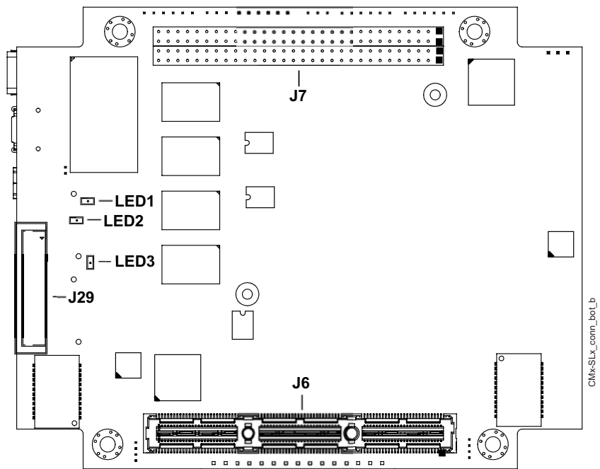
Figure 2-4: Header and Connector Locations (Bottom Side)
