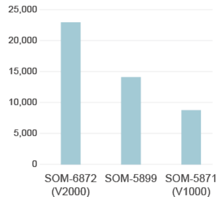
CPU PassMark
