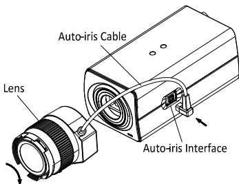
Figure 2-2 Installing the Lens
