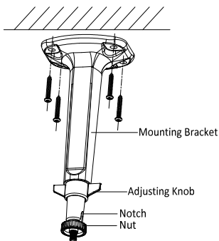
Figure 2-3 Installing the Mounting Bracket
