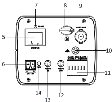
Figure 1-2 Interfaces on the Rear Panel
