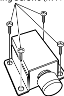
Self-Tapping Screws (M4 x 12)
