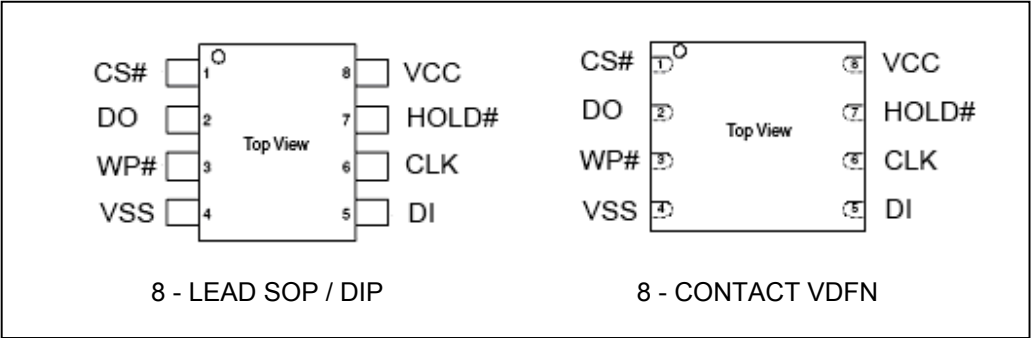
Figure.1 CONNECTION DIAGRAMS
