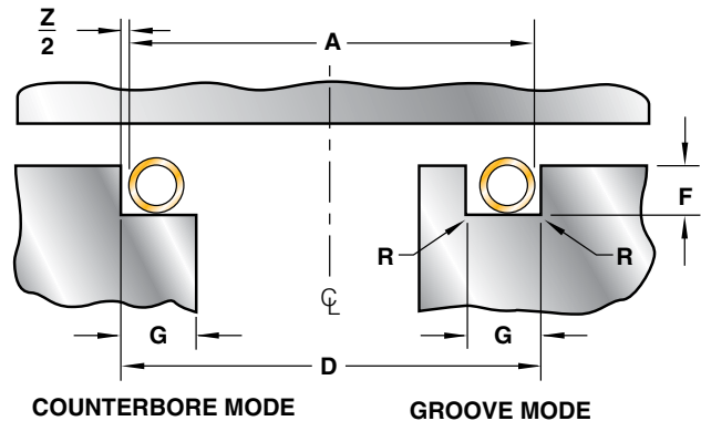
Cavity Dimensions
