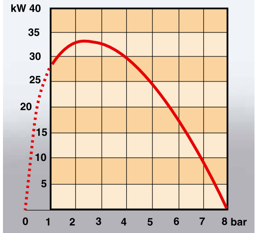
Adiabatic power requirement for a booster compressor with an absolute final pressure of 8 bar(a).
