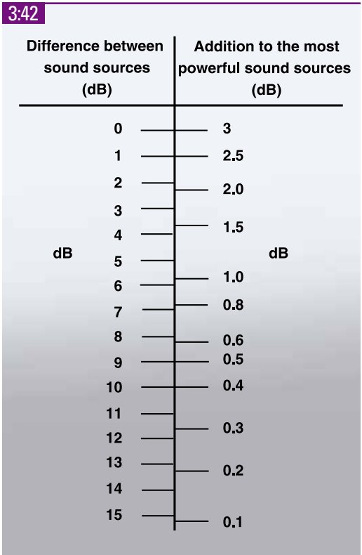
The nomogram defines how many dB shall be added to the highest sound level when adding two sound levels.
