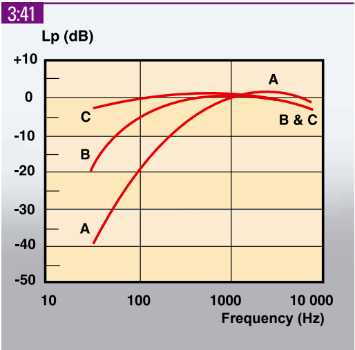
Frequency dependency of the different filters used to weight sound levels when measuring sound. Most common is the A-filter.
