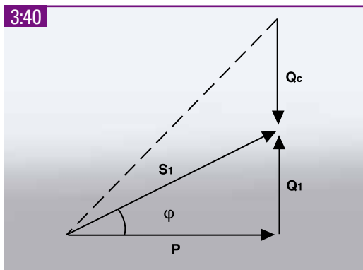
Reactive power Q_c is supplied to increase the motor power factor \cos(\varphi) to 1.
