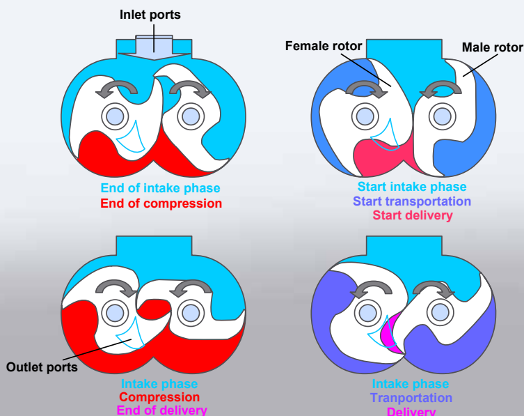
Compression principle of the double tooth compressor.
