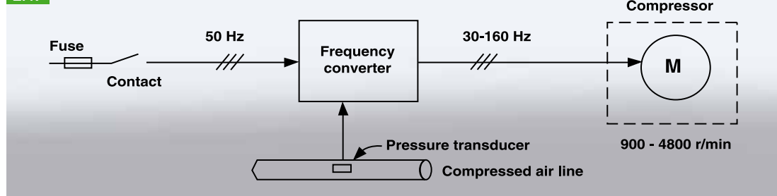
A system with a speed controlled compressor.
