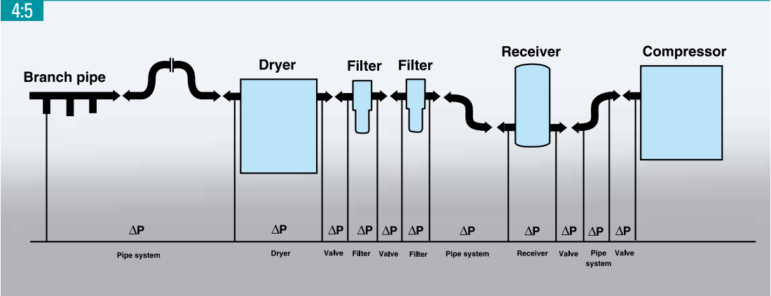
The pressure drop across different components in the network affects the requisite working pressure.
