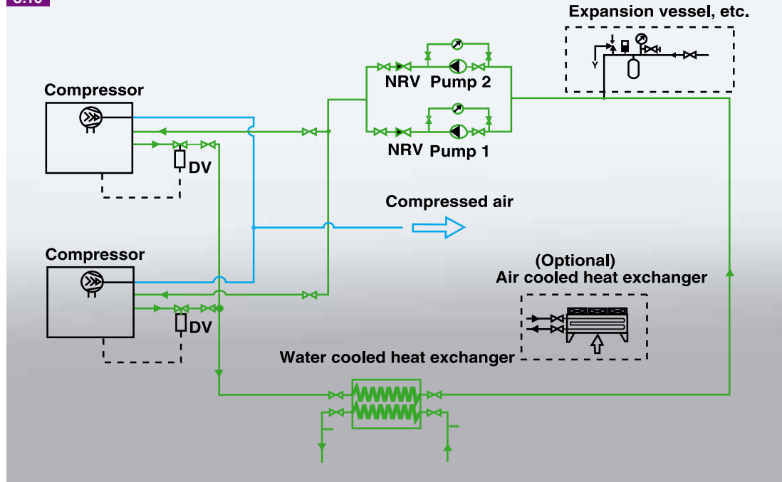
Schematic of a closed cooling system. The heat exchanger can be water cooled or air cooled.
