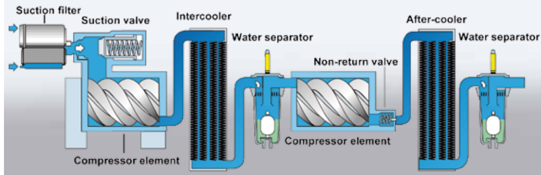
Oil-free screw compressor flow diagram.
