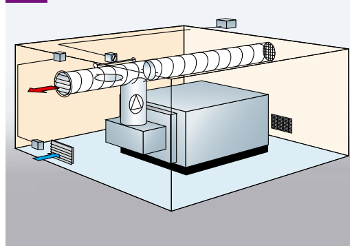
Energy recovery from an air-cooled compressor.
