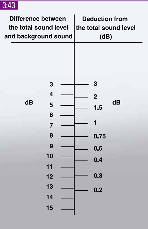
The nomogram defines how many dB shall be deducted from the total sound level at different background sound levels in order to estimate the net sound level.
