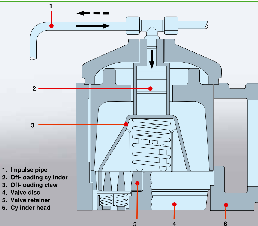
Off-loading device for a piston compressor.
