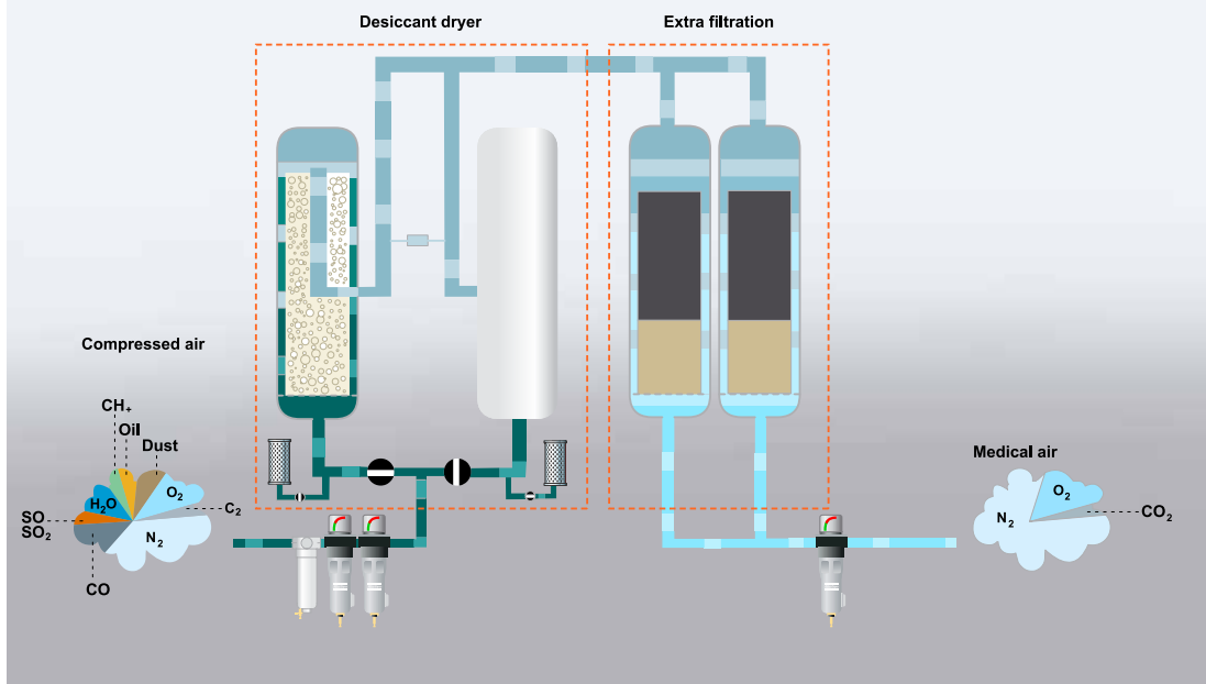
Schematic of an installation that delivers medical air.
