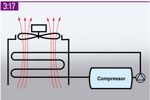
A basic air heater (air cooled heat exchanger) can be found in closed cooling systems for cooling liquids such as water/glycol, oil, etc. In aggressive environments or with aggressive liquids stainless steel or titanium coolers are used.
