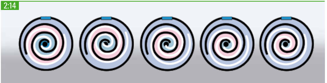
Compression principle of a scroll compressor.
