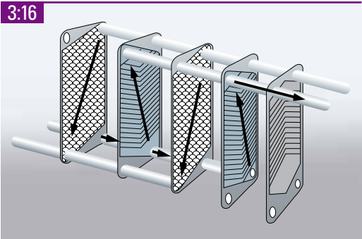
Illustration of a flat heat exchanger. Flat heat exchangers are easy to clean, which makes it possible to indirectly cool the compressor using lake water or stream water.
