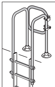
Long exit rail (with a safety barrier)
