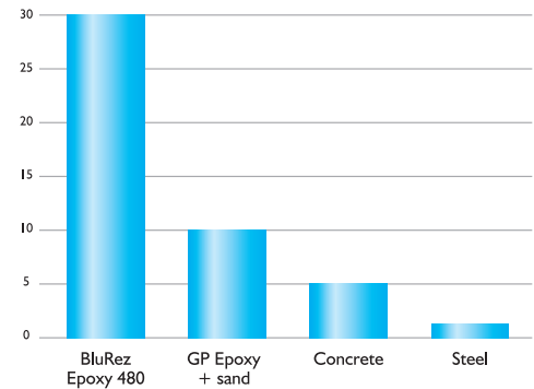
CHARACTERISTIC VIBRATION DAMPING CAPABILITY
