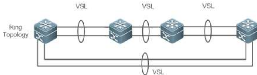
Figure 8-9 Ring Topology
