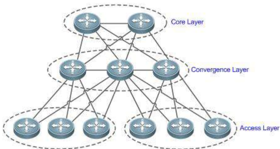
Figure 6-2 Hierarchical Topology
