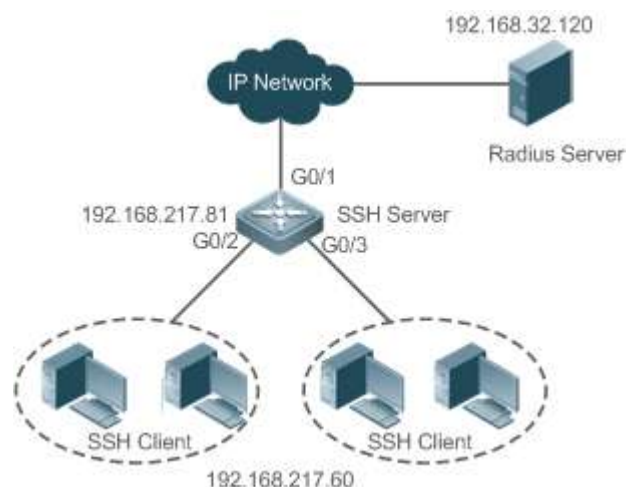
Figure 9-3 Networking Topology of SSH AAA Authentication
