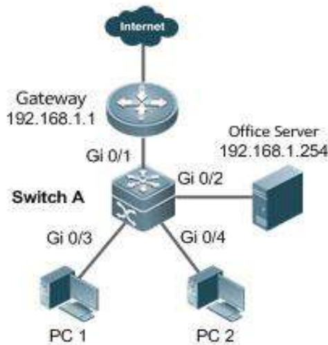
Figure 16-1 Typical Topology of Gateway-targeted ARP Spoofing Prevention
