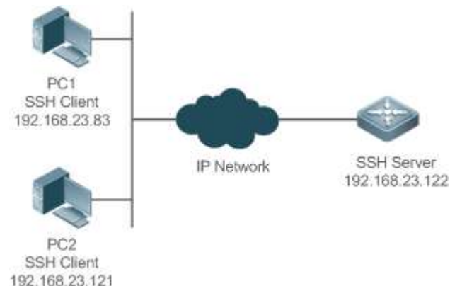
Figure 9-2 Networking Topology of SSH Local Line Password Authentication
