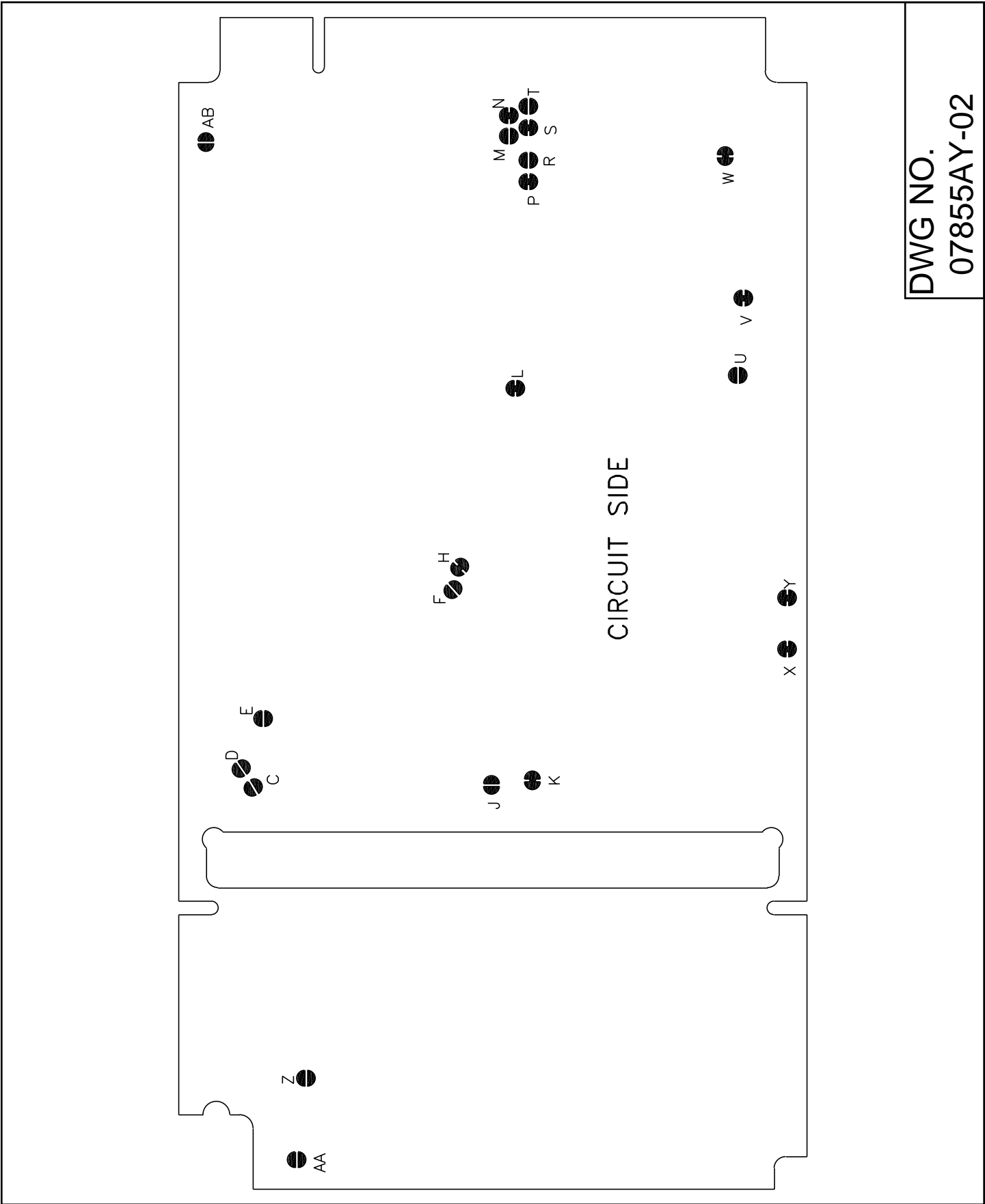
PCBA DWG, 2003B, 4 1/2 DIGIT DPVM - SOLDERSWITCHES
