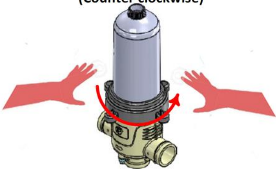
Step one Release the Nut lock ring (Counter clockwise)
