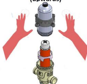
Step two Remove The filter cup (upwards)
