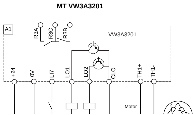
Connection diagram for logic I/O option card (MT-VW3A3201)
