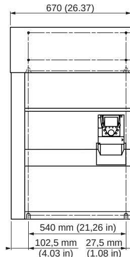
I MT4300 to MT4400 with braking unit
