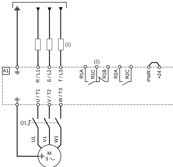
Diagram with disconnect switch
