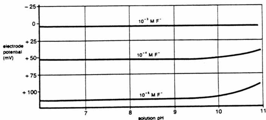
Figure 5 Electrode response in alkaline solution
