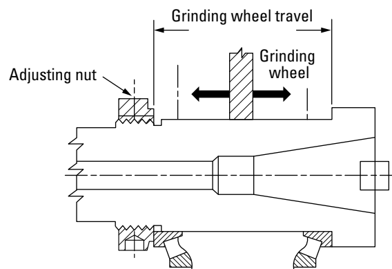
Fig. 115. Grinding of inner ring shaft and backing shoulders.
