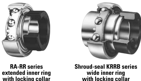
Fig. 13. Self-locking (eccentric) collar.
