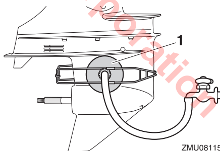
1. Flushing attachment
