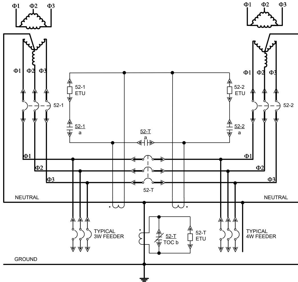
Figure 9: Single point grounding scheme
