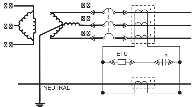
Figure 12: MDGF sensor arrangement for drawout WL breakers
