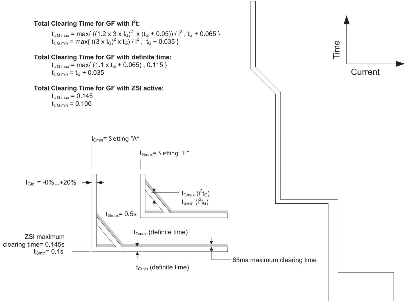
Figure 13: WL Ground Fault Time-Current Characteristics
