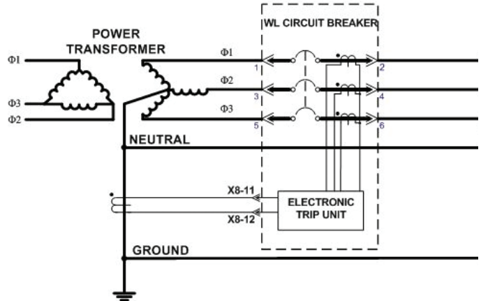
Figure 6: Direct ground current sensing – 3-wire or 4-wire system
