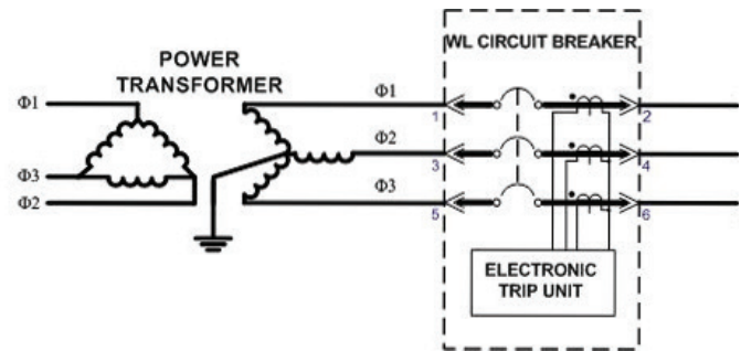
Figure 2: Residual ground current sensing – 3-wire system
