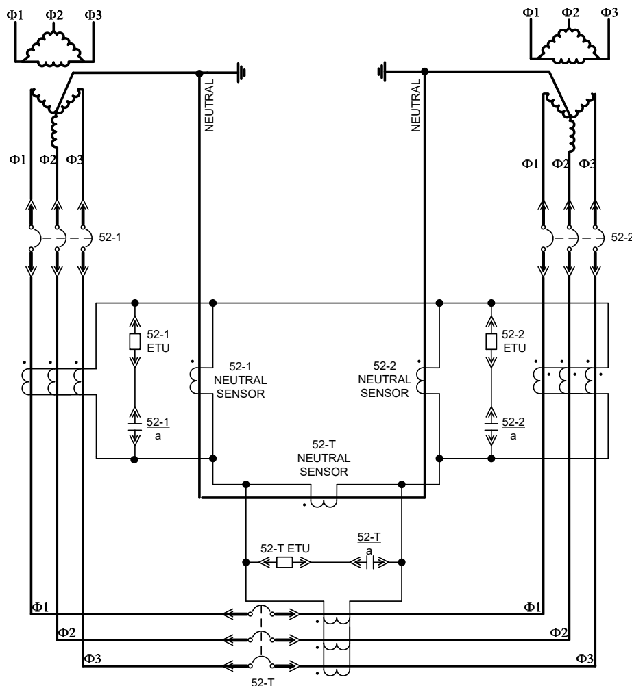
Figure 10: Modified differential ground fault sensing scheme
