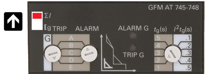
Figure 1: WLGFM48 Ground fault module (Residual sensing setting)
