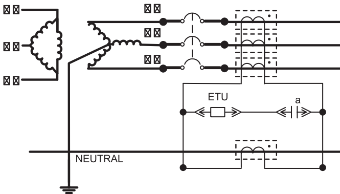
Figure 11: MDGF Sensor arrangement for fixed-mounted WL breakers
