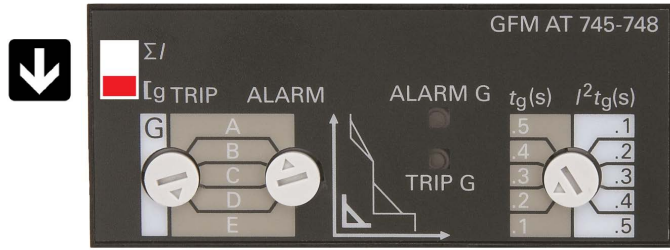
Figure 8: WLGAT748 Ground fault module (direct sensing setting)
