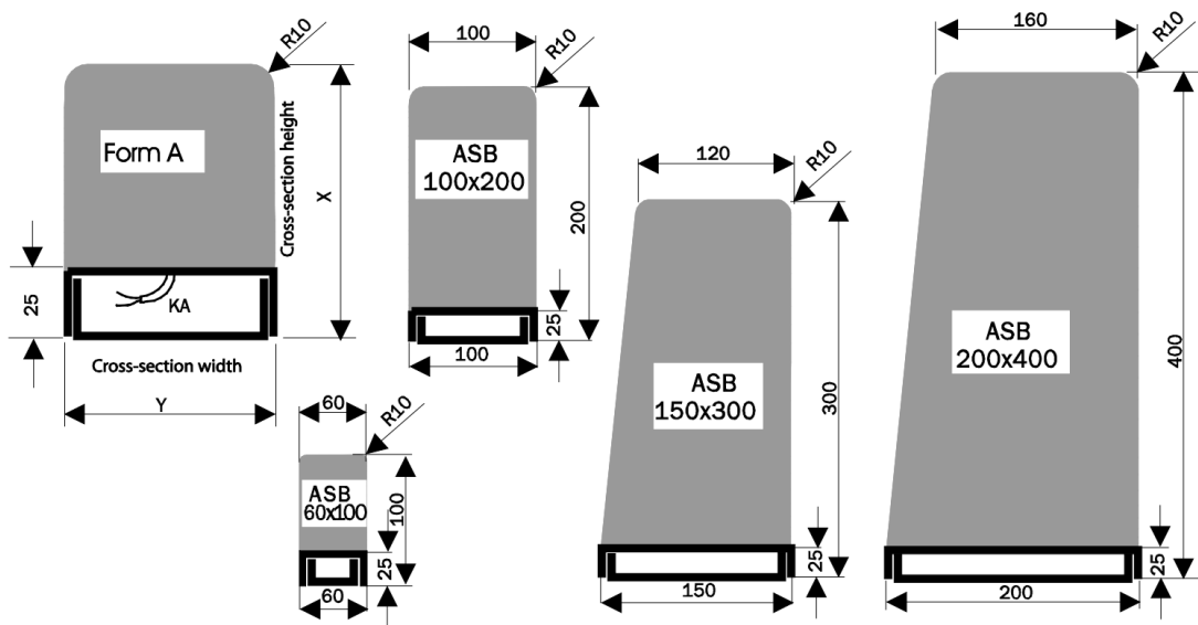
Figure 6: Bumper dimensions
