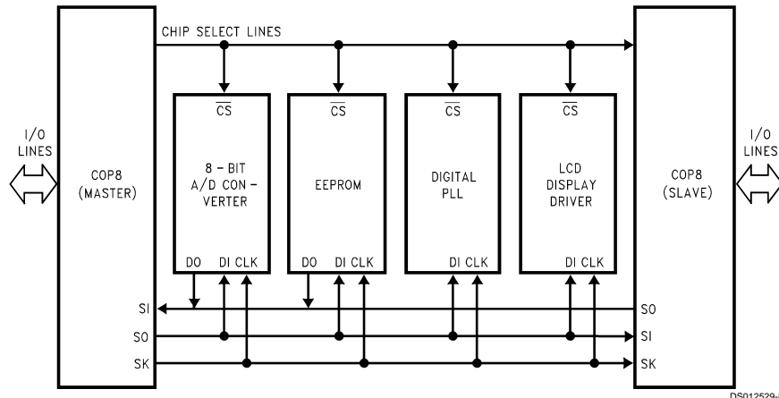
FIGURE 7. MICROWIRE/PLUS Application
