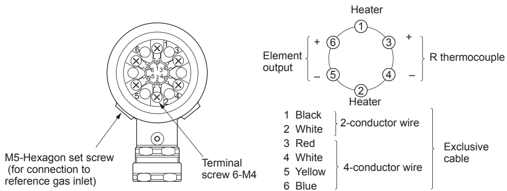
External terminal of detector & wire colors
