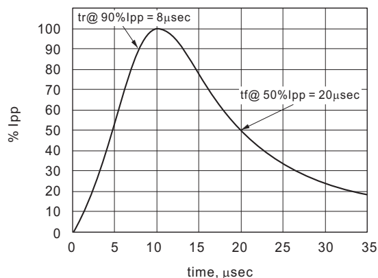
Fig.5 8x20µsec Surge Waveform
