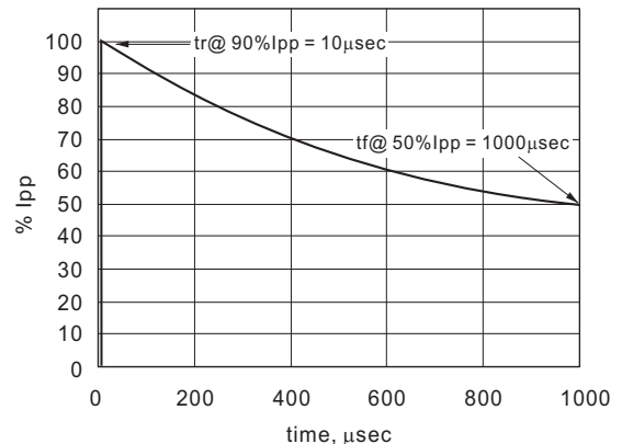
Fig.6 10x1000µsec Waveform
