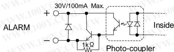
Fig.13. ALARM Output
