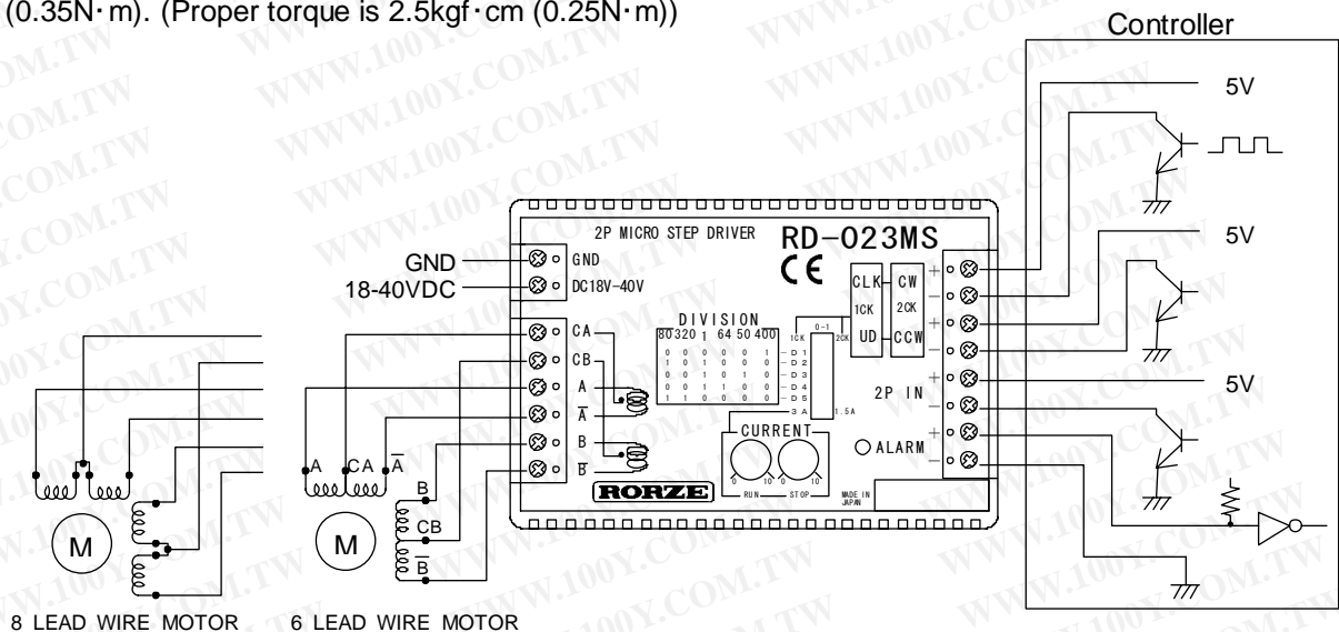
Fig.14. Wiring Diagram
