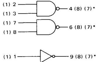
MC862G/MC962G MC863G/MC963G Dual 2-Input NAND Gate Plus Inverter
