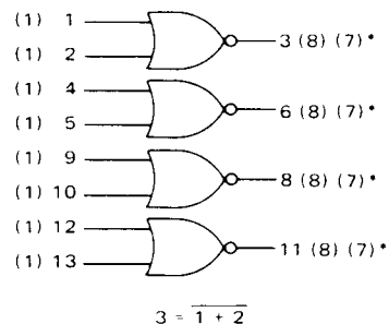
MC1810/MC1910 MC1811/MC1911 Quad 2-Input NOR Gate
