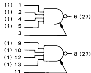
MC844/MC944 Expandable Dual 4-Input Power NAND Gate
