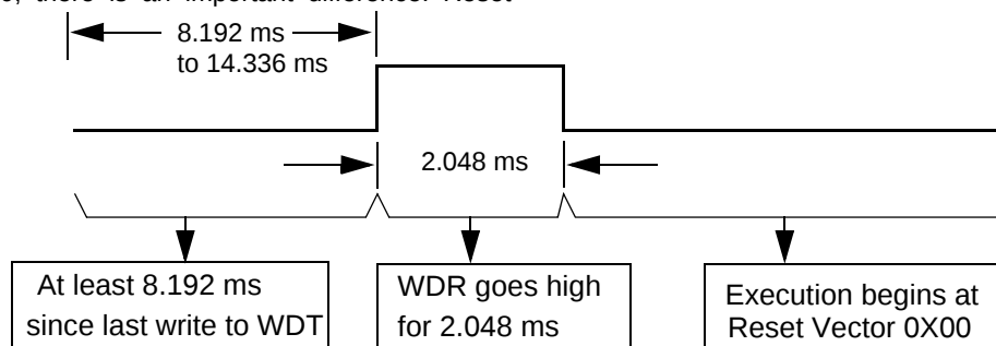
Figure 3. Watch Dog Reset (WDR)
