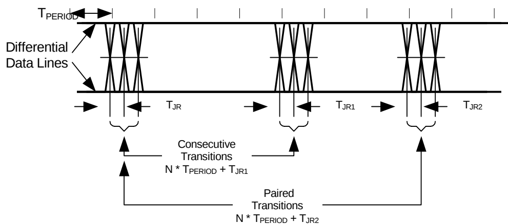
Figure 10. Receiver Jitter Tolerance
