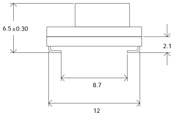
Figure 57. Side View
