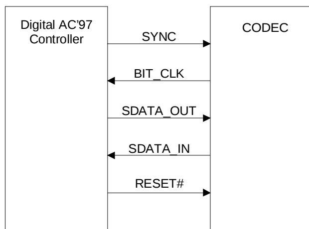
Figure 7. AC-link Connections
