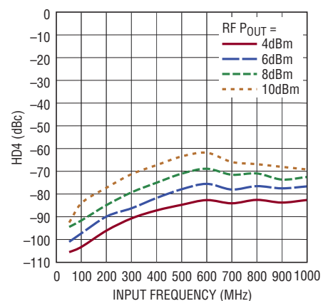
HD4 vs Input Frequency Over P_{OUT}
