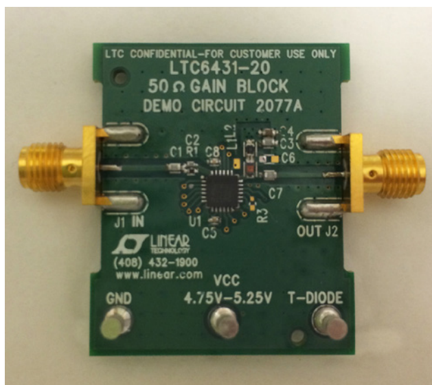
Figure 3. Demo Board
