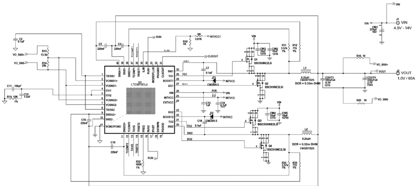
Figure 24. Dual Phase 1.0V, 60A Power System with Ultralow DCR Sensing
