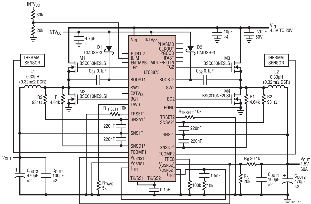
Figure 17. High Efficiency Dual Phase 400kHz, 1.5V/60A Step-Down Converter with Optional Thermal Balancing
