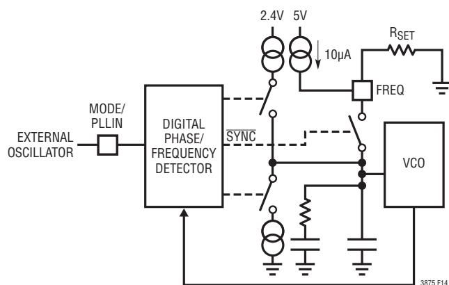
Figure 14. Phase-Locked Loop Block Diagram
