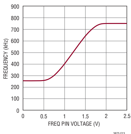
Figure 13. Relationship Between Oscillator Frequency and Voltage at the FREQ Pin
