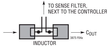
Figure 4a. Sense Lines Placement with Inductor DCR
