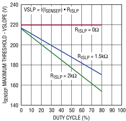
I SENSEP Maximum Threshold - VSLP vs Duty Cycle (Programming Slope Compensation)
