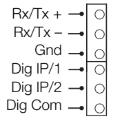
F Ethernet/Modbus and Digital Input
