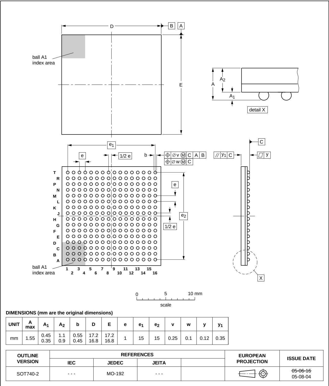
Fig 49. Package outline LBGA256 package
