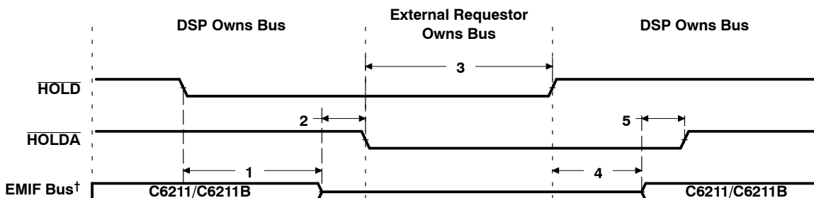
Figure 29. HOLD/HOLDA Timing
