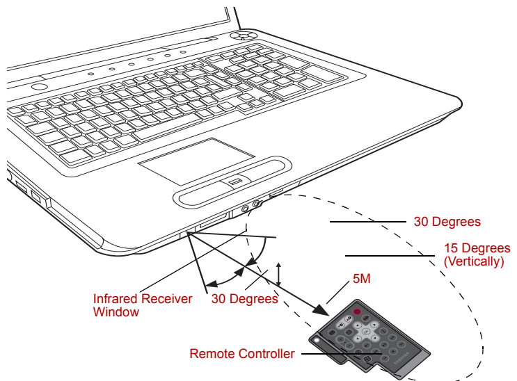
Operational range of the remote controller
