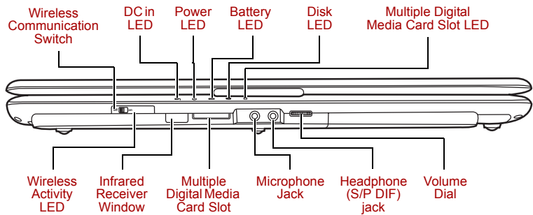
Front of the computer with display closed
