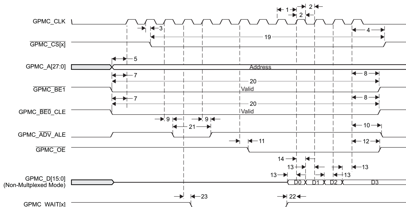
Figure 8-20. GPMC Non-Multiplexed NOR Flash - 14x16-bit Synchronous Burst Read (GPMCFCLKDIVIDER = 0)
