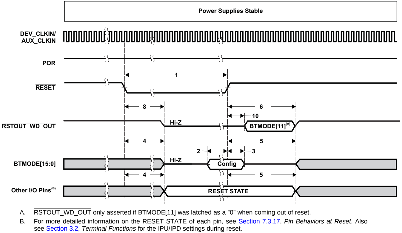
Figure 7-3. Warm Reset ( \overline{\text{RESET}} ) Timing
