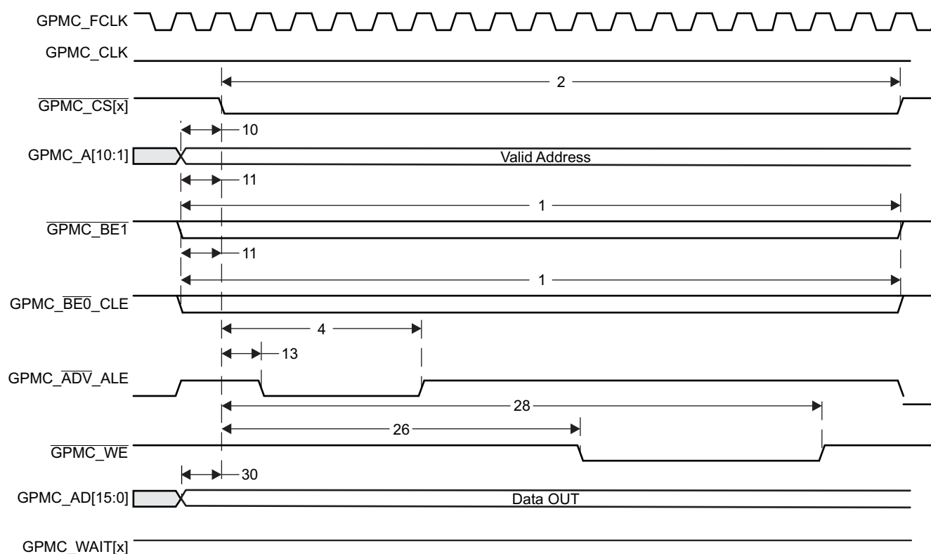
Figure 8-28. GPMC/Non-Multiplexed NOR Flash - Asynchronous Write - Single Word Timing
