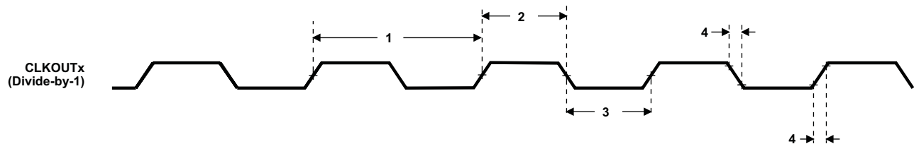
Figure 7-13. CLKOUTx Timing
