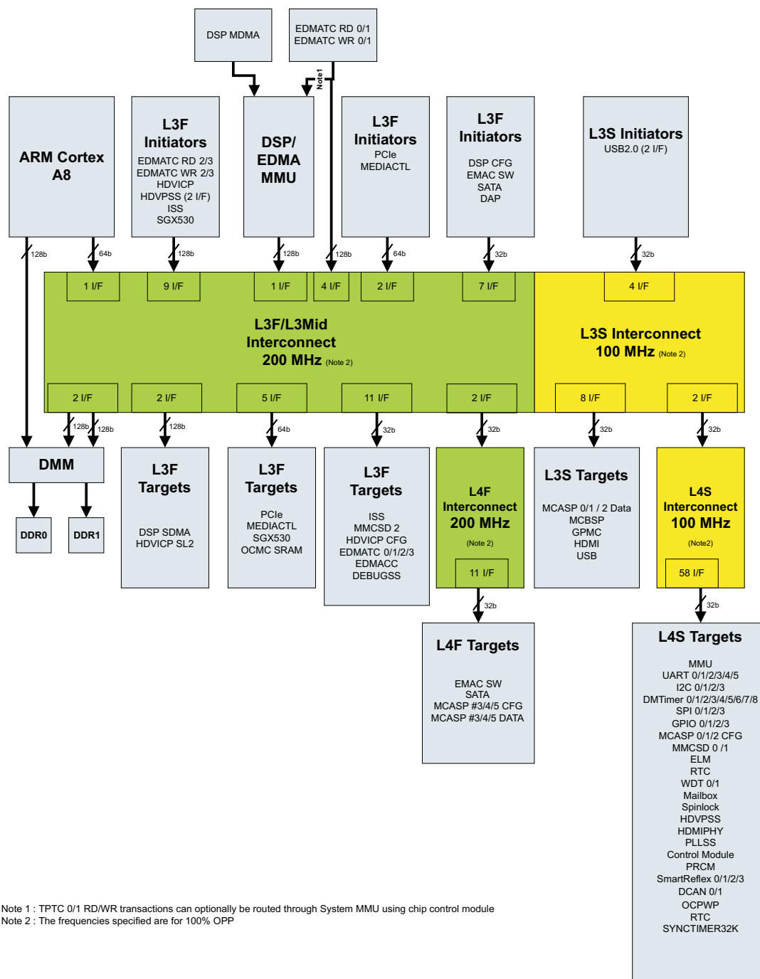
Figure 5-1. System Interconnect
