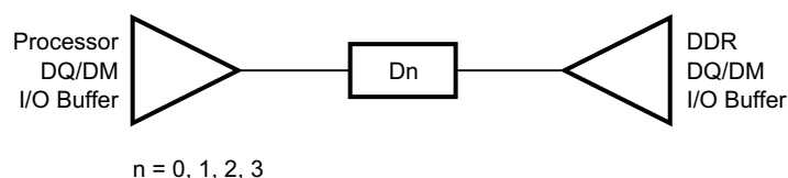
Figure 8-75. DQ/DM Topology
