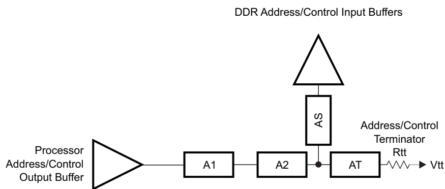
Figure 8-71. ADDR_CTRL Topology for One DDR3 Device
