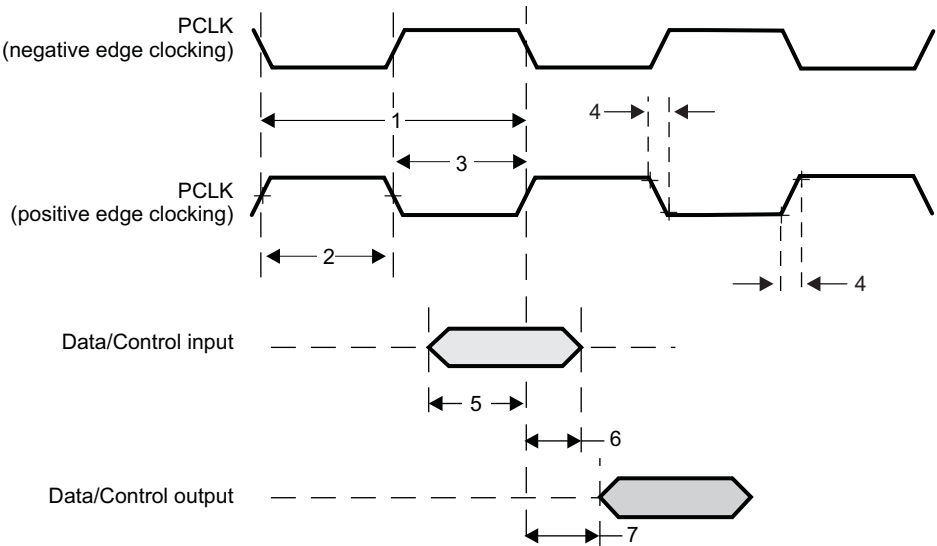
Figure 8-43. ISSCAM Timings
