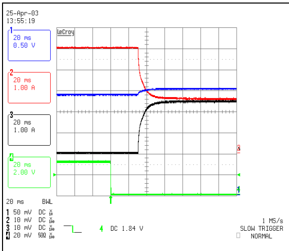
Start-up with Back-biased Voltage (2.4V) and 5A Load. Ch. 1: Vo Ch. 2: Ibias Ch. 3: Io Ch. 4: ON/OFF
