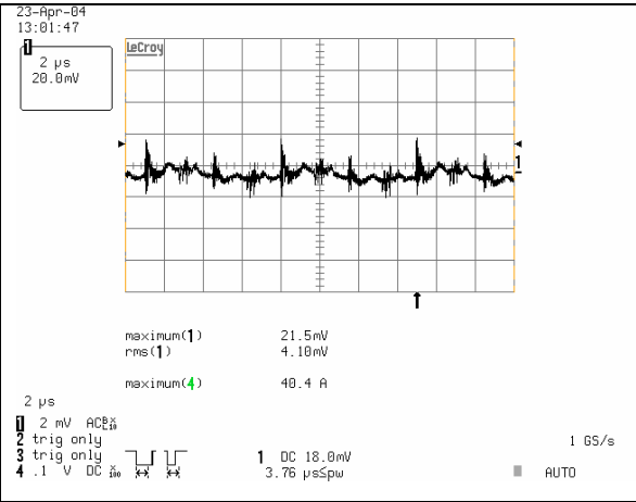
Typical Output Ripple at 48V Input and Full Load at Ch. 1: Vo
