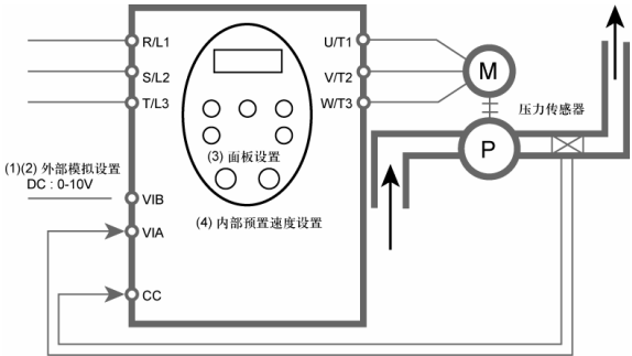
反馈信号 (1) DC: 4-20mA (2) DC: 0-10V
