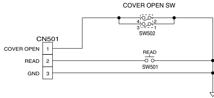
KX-FM383CN : SENSOR BOARD (PCB5)
