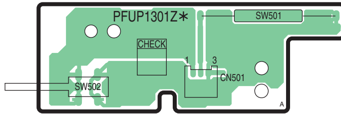
KX-FM383CN : SENSOR BOARD(PCB5)
