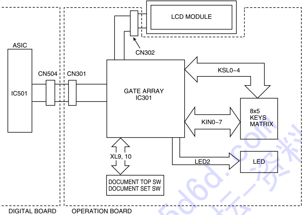
KX-FP383CN : OPERATION BOARD BLOCK DIAGRAM
