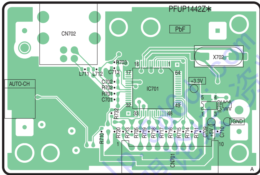
KX-FM383CN : USB BOARD (PCB6) : COMPONENT VIEW
