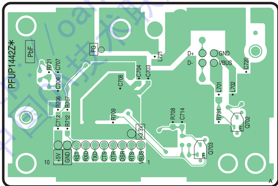
KX-FM383CN : USB BOARD (PCB6) : BOTTOM VIEW
