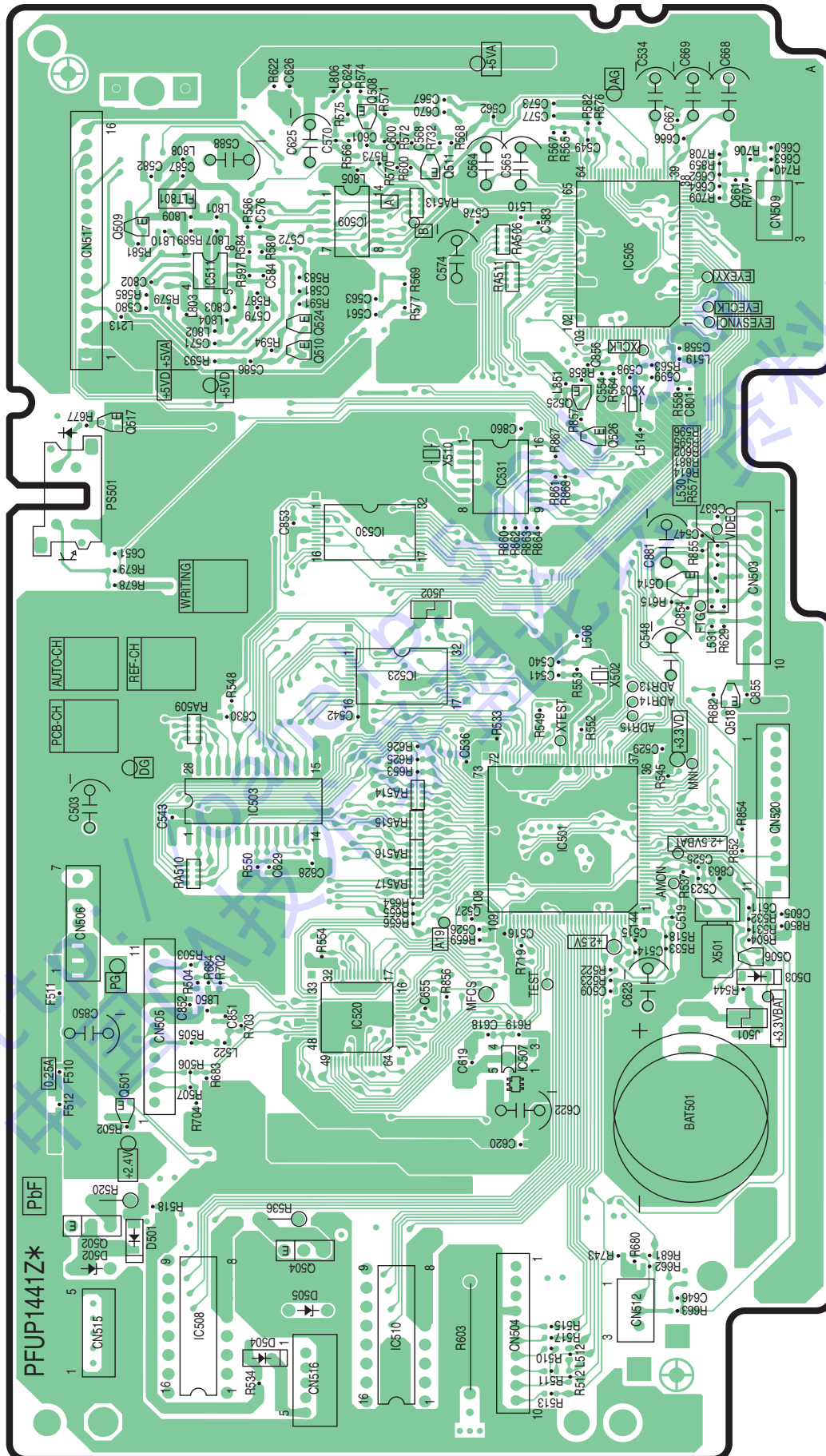
KX-FM383CN : DIGITAL BOARD (PCB1) : COMPONENT VIEW
