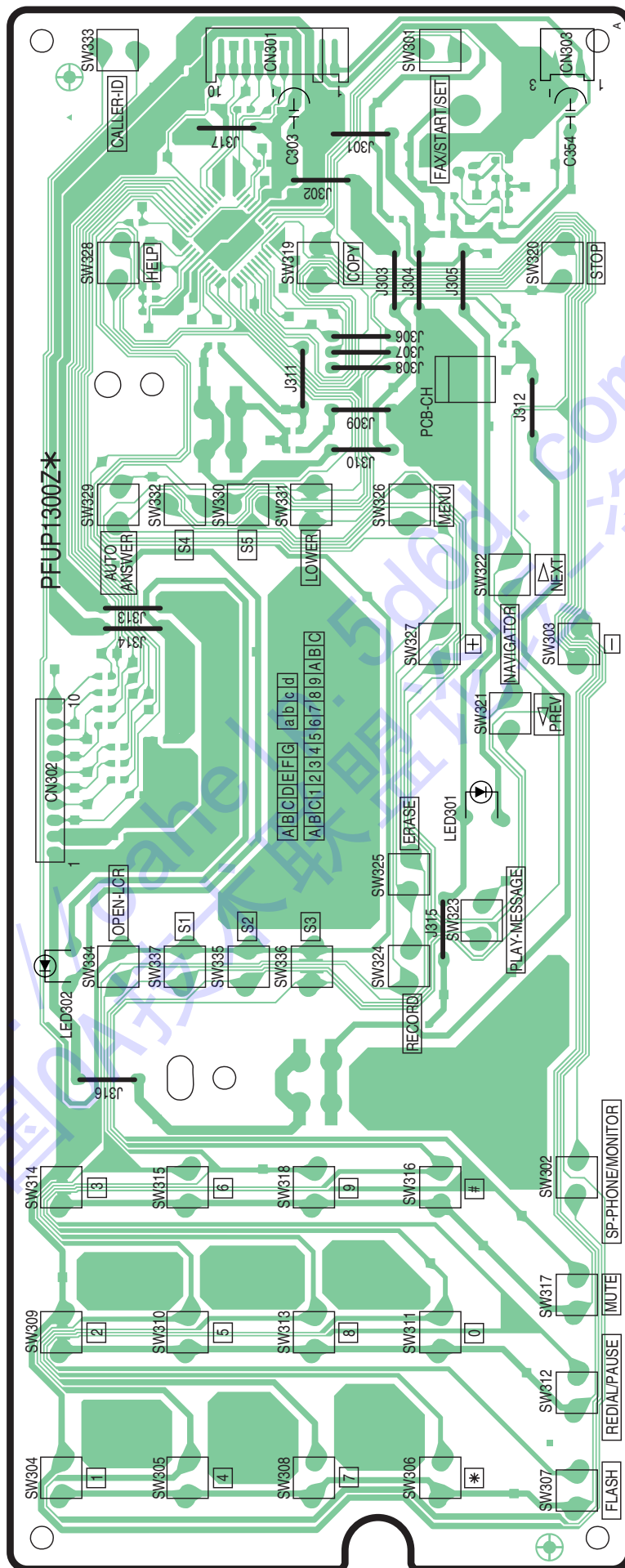
KX-FM383CN : OPERATION BOARD(PCB3) : COMPONENT VIEW
