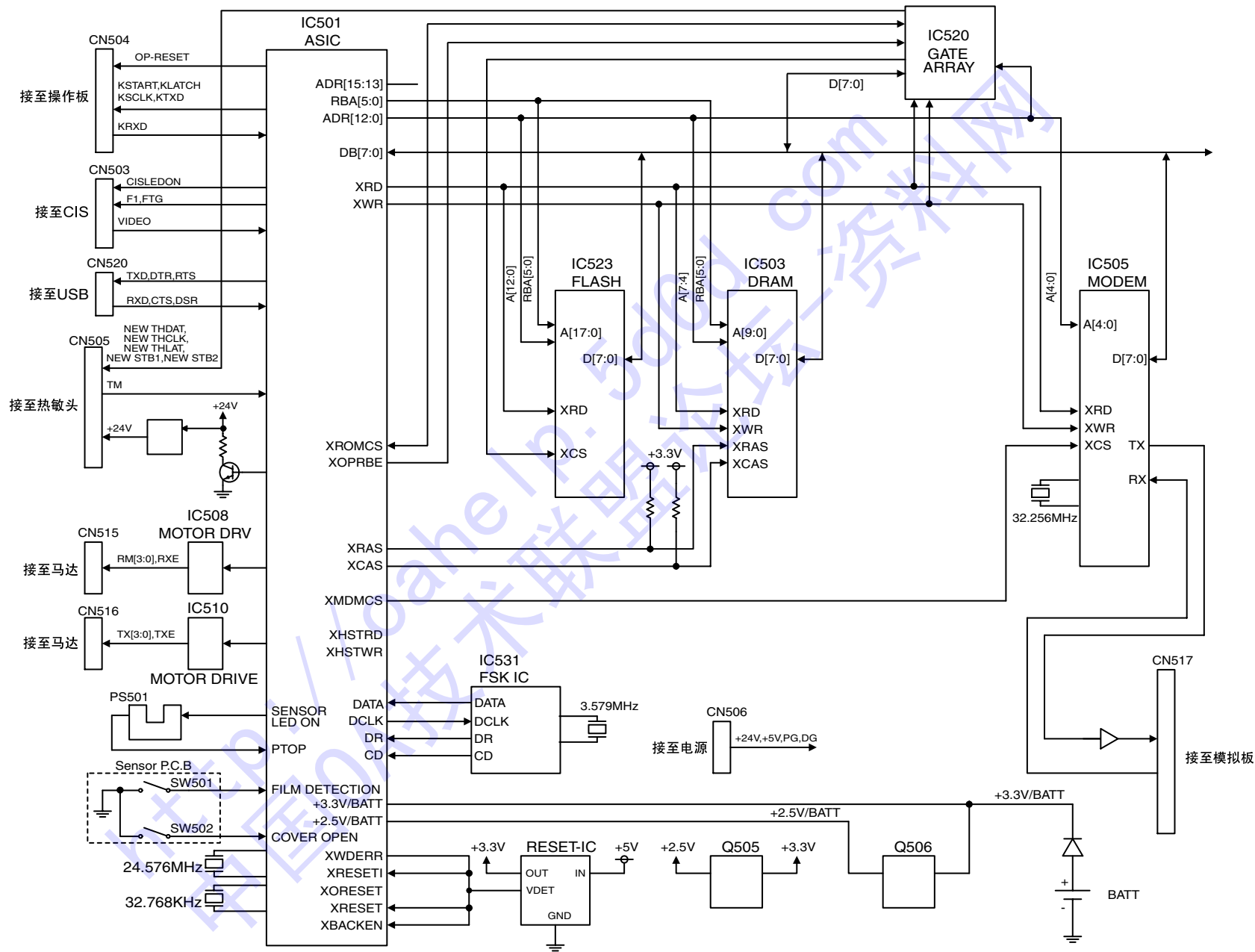
KX-FM383CN : DIGITAL BOARD BLOCK DIAGRAM
