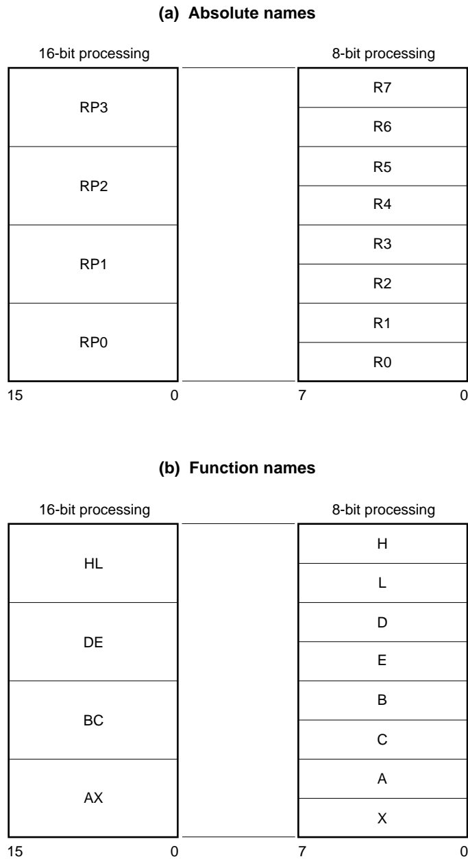
Figure 3-18. General-Purpose Register Configuration
