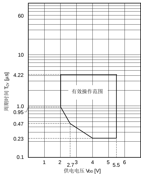
T_{CY} VS. V_{DD} (高速内部振荡器时钟)
