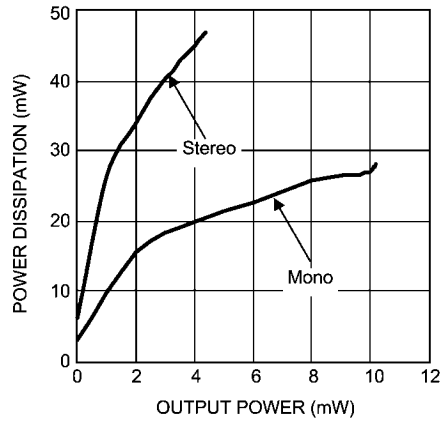
Power Dissipation vs Output Power V_{DD} = 1.6V , R_L = 16 , f = 1kHz
