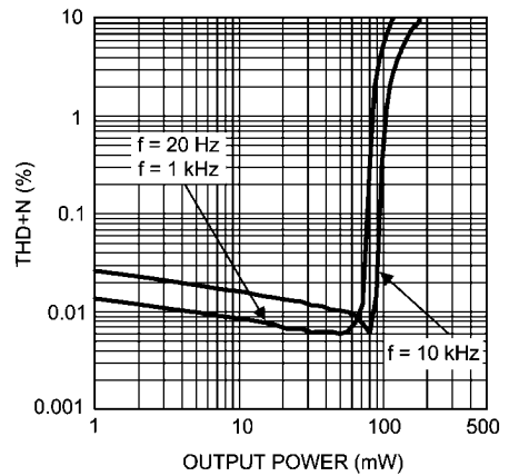
THD+N vs Output Power V_{DD} = 3V , R_L = 32 , One channel
