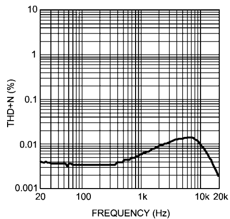
THD+N vs Frequency V_{DD} = 3V , R_L = 32 , One channel, P_O = 50mW
