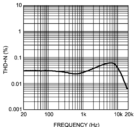
THD+N vs Frequency V_{DD} = 1.6V , R_L = 16 , Stereo, P_O = 3mW
