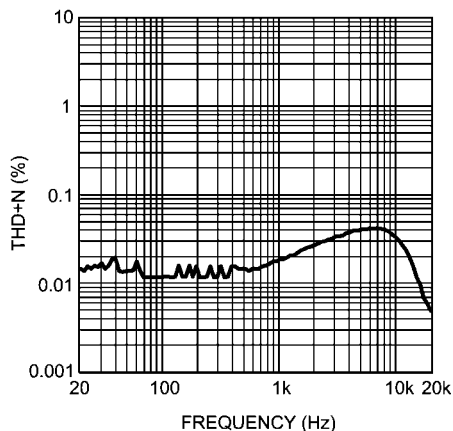
THD+N vs Frequency V_{DD} = 3V , R_L = 16 , Stereo, P_O = 25mW
