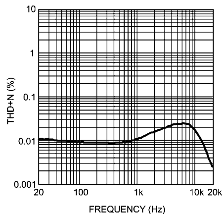
THD+N vs Frequency V_{DD} = 3V , R_L = 16 , One channel, P_O = 60mW
