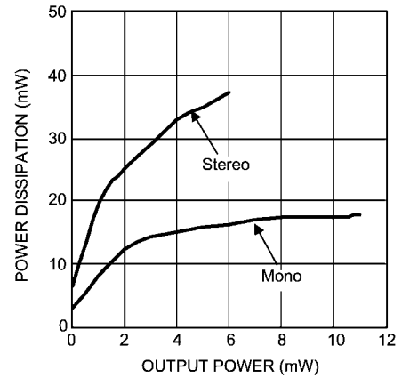
Power Dissipation vs Output Power V_{DD} = 1.6V , R_L = 32 , f = 1kHz
