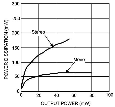
Power Dissipation vs Output Power V_{DD} = 3V , R_L = 32 , f = 1kHz
