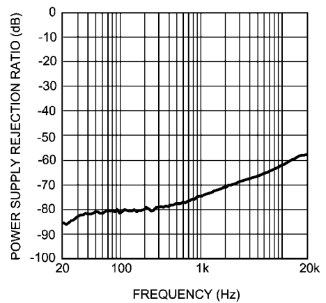
PSRR vs Frequency V_{DD} = 1.6V , R_L = 32
