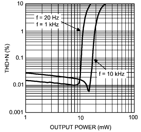
THD+N vs Output Power V_{DD} = 1.6V , R_L = 32 , One channel
