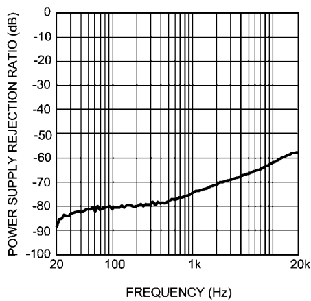
PSRR vs Frequency V_{DD} = 1.6V , R_L = 16
