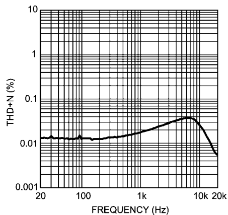
THD+N vs Frequency V_{DD} = 1.6V , R_L = 32 , Stereo, P_O = 3mW
