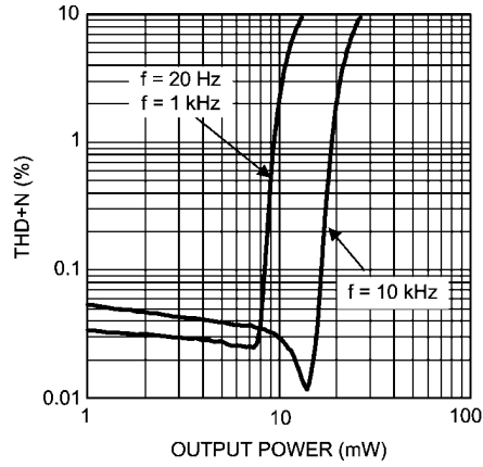
THD+N vs Output Power V_{DD} = 1.6V , R_L = 16 , One channel
