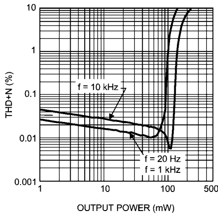
THD+N vs Output Power V_{DD} = 3V , R_L = 16 , One channel
