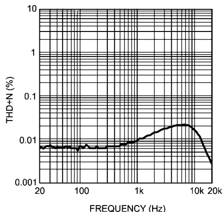
THD+N vs Frequency V_{DD} = 3V , R_L = 32 , Stereo, P_O = 25mW
