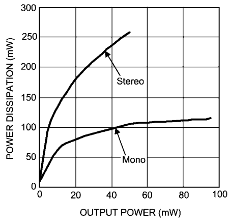
Power Dissipation vs Output Power V_{DD} = 3V , R_L = 16 , f = 1kHz
