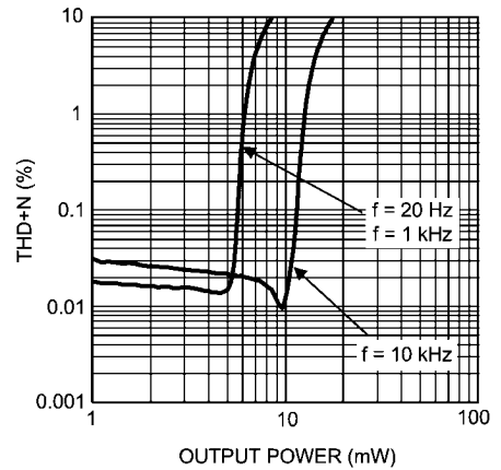
THD+N vs Output Power V_{DD} = 1.6V , R_L = 32 , Stereo
