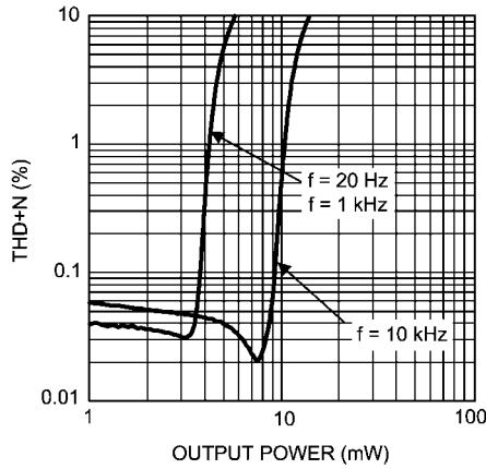
THD+N vs Output Power V_{DD} = 1.6V , R_L = 16 , Stereo
