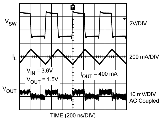
FIGURE 6. Typical PWM Operation
