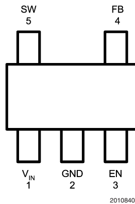
FIGURE 3. TopView SOT23-5 Package NS Package Number MF05A
