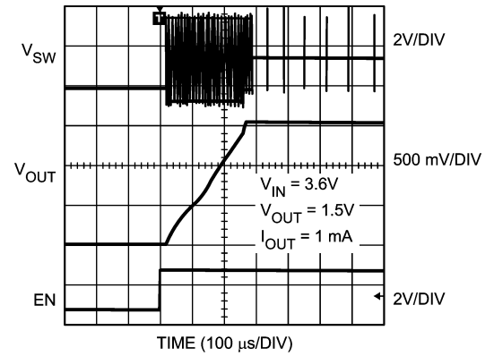
Start Up into PFM Mode (Output Current= 1mA)
