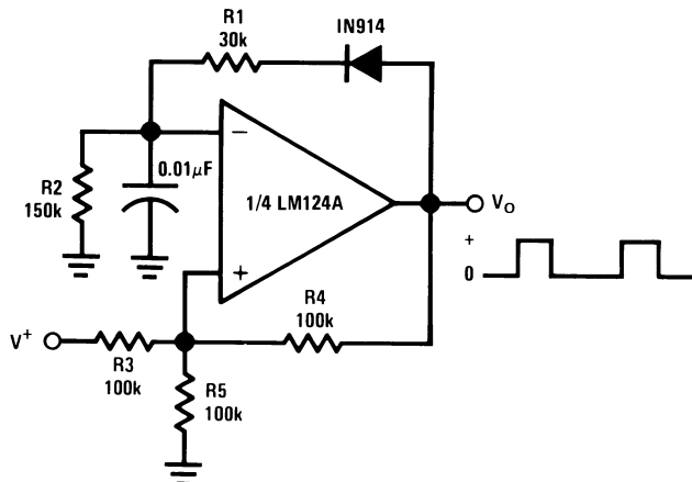
Pulse Generator
