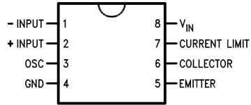
Dual-In-Line Package
