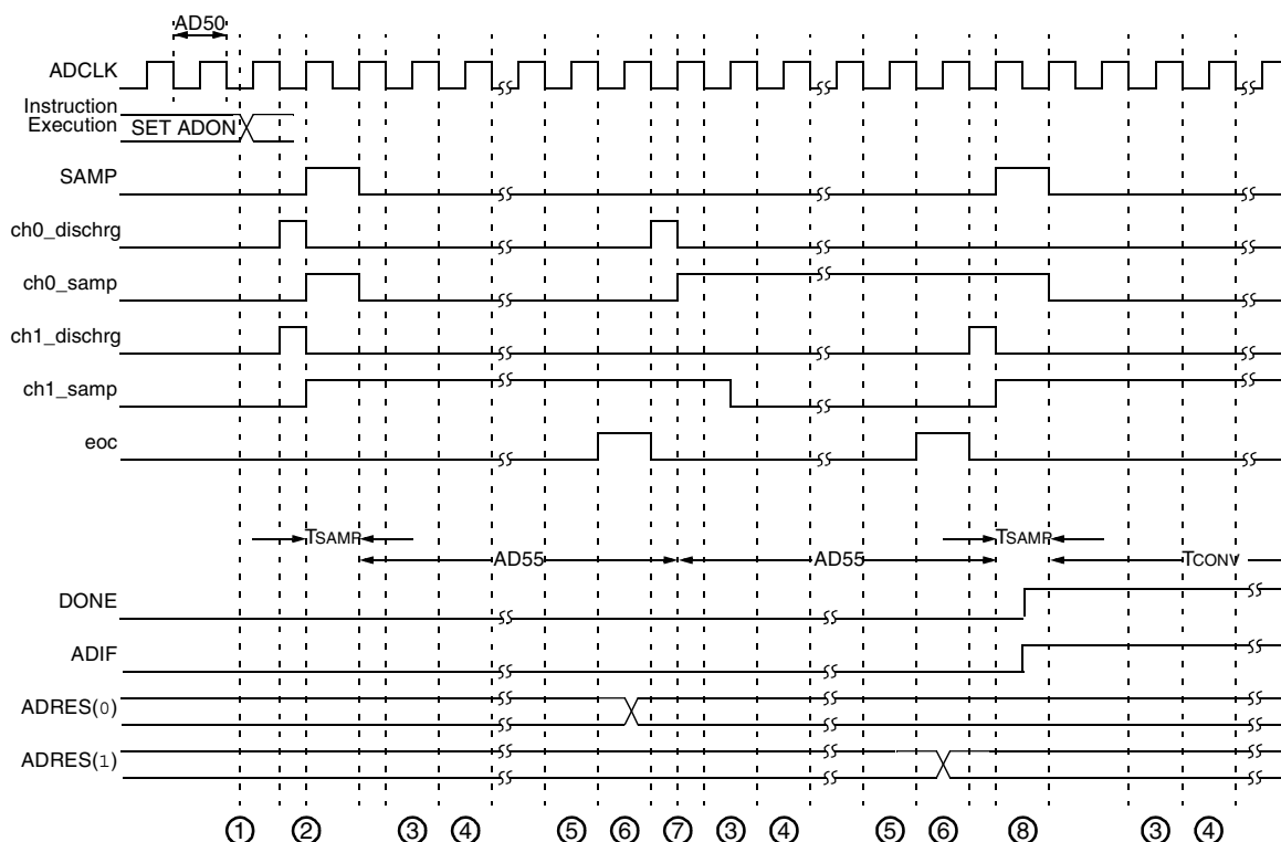
FIGURE 24-26: 10-BIT HIGH-SPEED A/D CONVERSION TIMING CHARACTERISTICS (CHPS = 01, SIMSAM = 0, ASAM = 1, SSRC = 111, SAMC = 00001)
