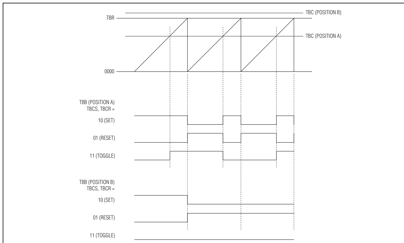
Figure 13. Up-Count PWM Mode
