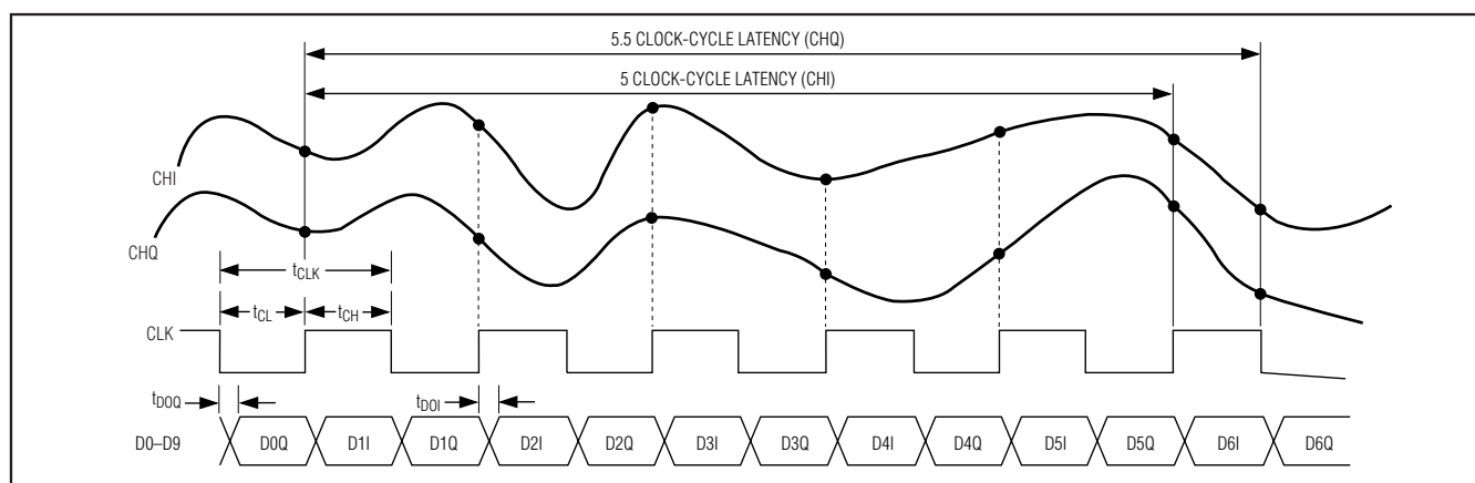
Figure 11. Receive ADC System Timing
