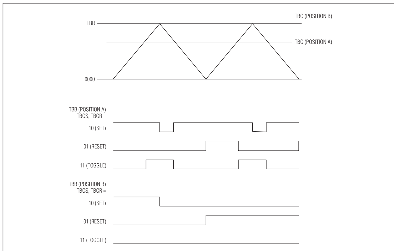
Figure 14. Up/Down Count PWM Mode
