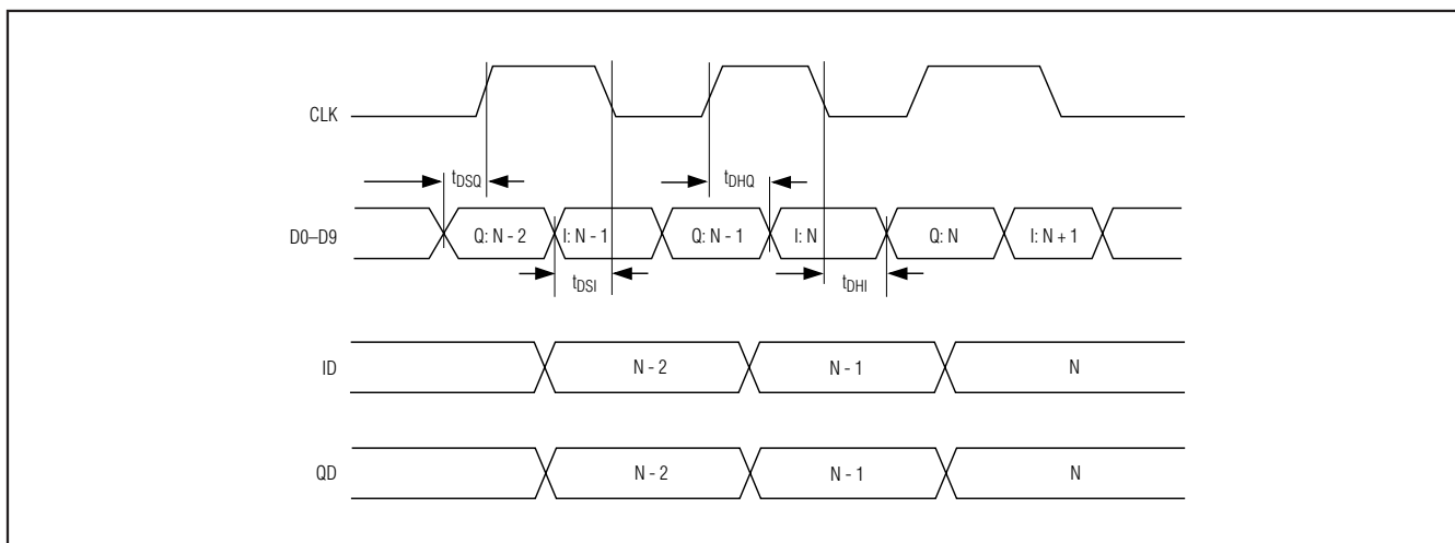
Figure 12. Transmit DAC System Timing
