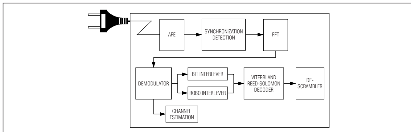
Figure 7. OFDM Receive Path
