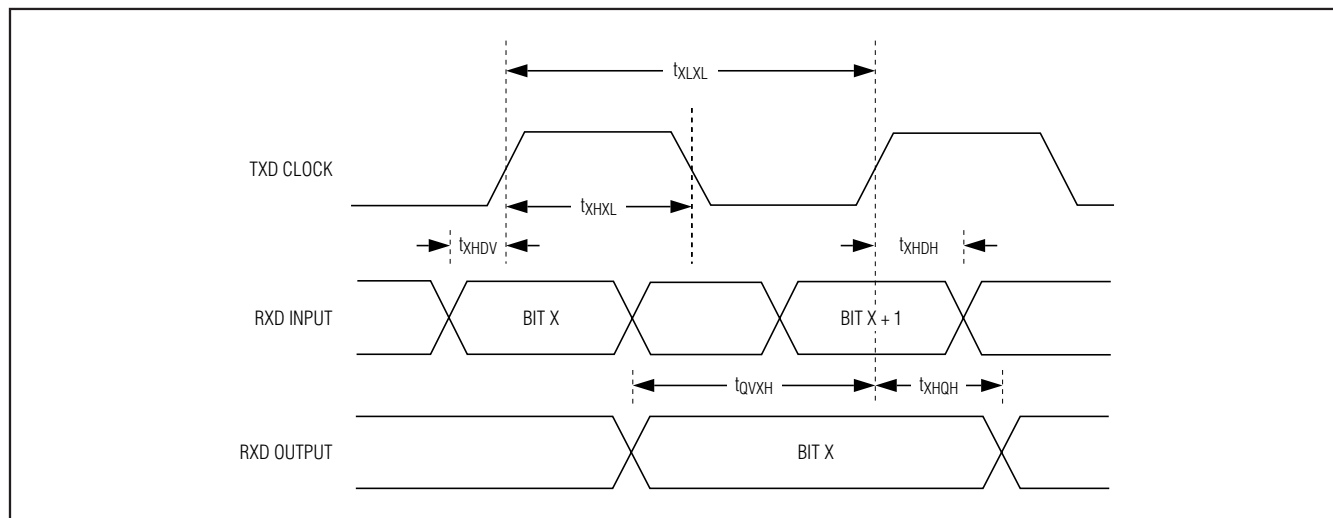
Figure 1. UART Timing Diagram for Synchronous Mode (Mode 0)
