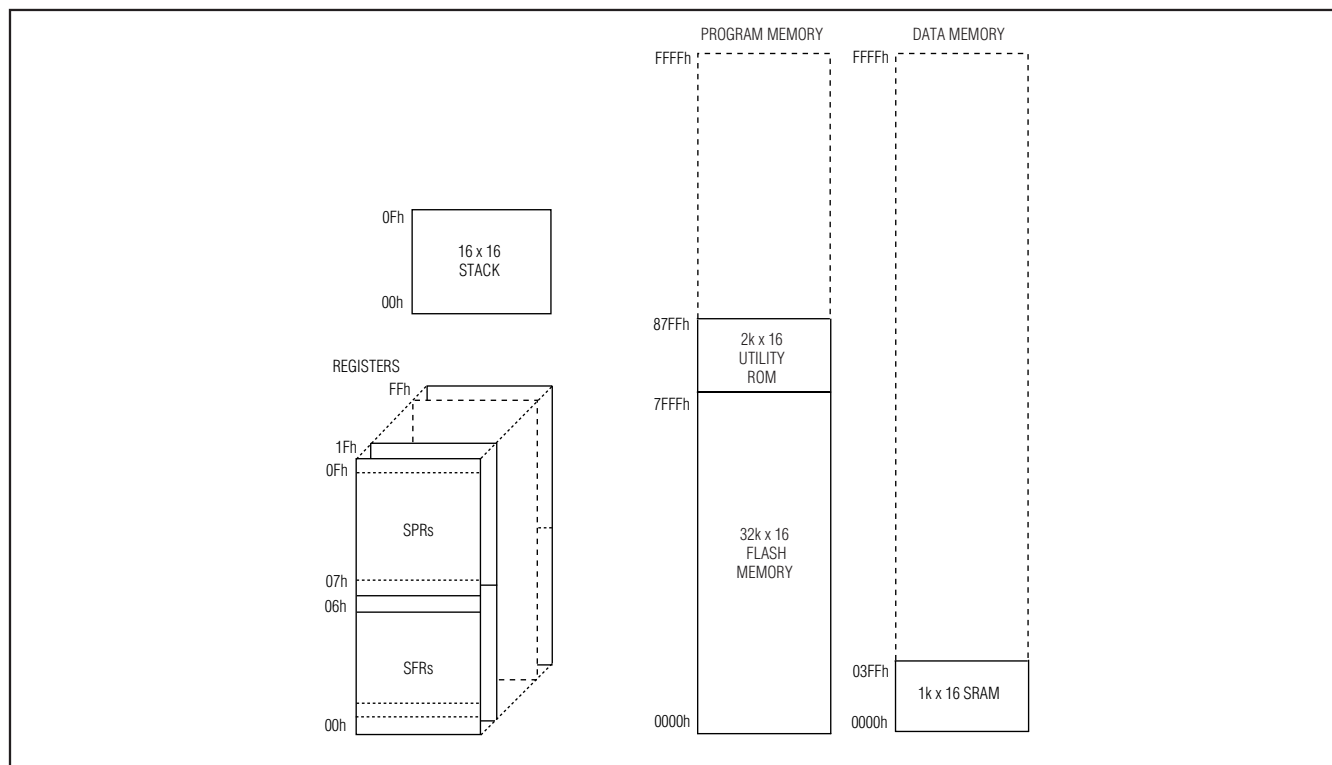
Figure 8. Memory Map
